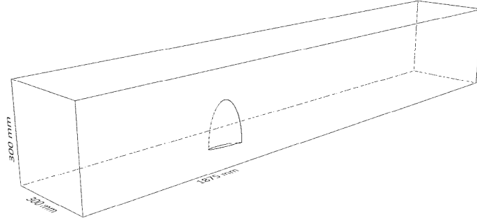
Figure 1: Computational domain, similar to the test section of the cavitation tunnel at the TU Delft. The flow is from left to right.
