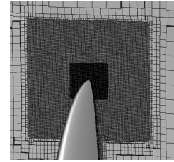
Figure 4: Grid refinement in the tip vortex region near the tip of the wing.
