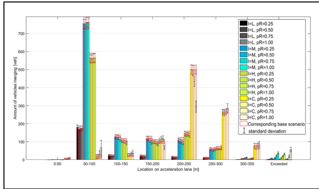
Figure 3. Merging location distribution. Note: I = intensity; L = low (free flow); M = medium (free flow); H = high (free flow); C = congestion; pR = penetration rate.
