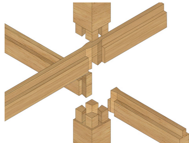
Solid wood structure
