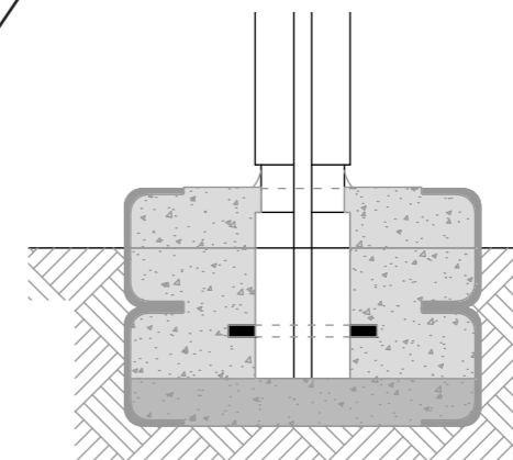
Concrete foundation
