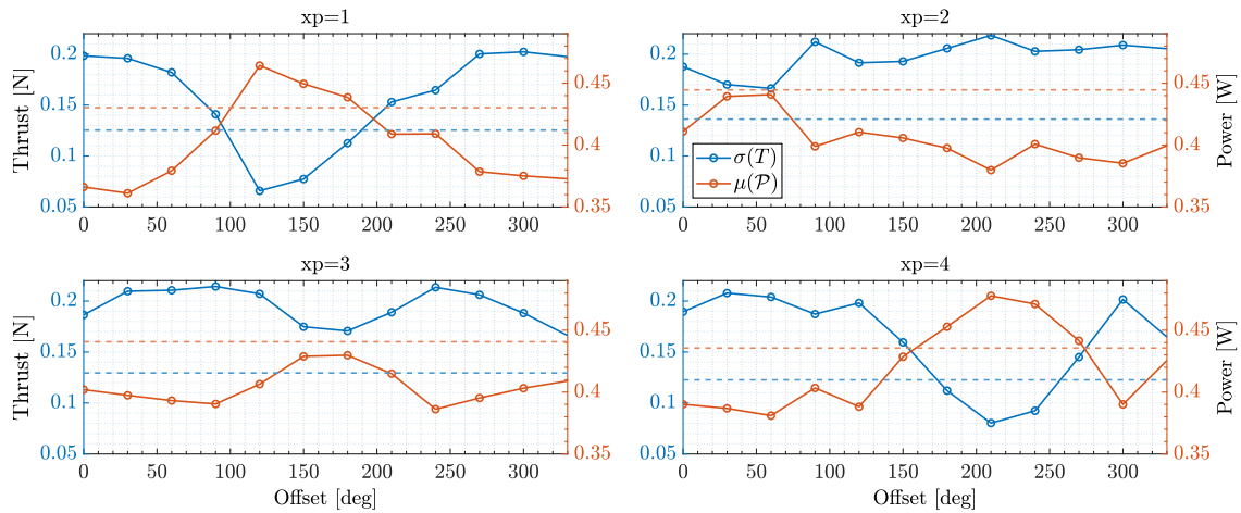
Figure 4: Power production of T2 overlaid with the thrust, for experiments 1 to 4. Each figure displays the results obtained in the respective experiment cycle. The baseline periodic DIC case is indicated by horizontal dashed lines.
