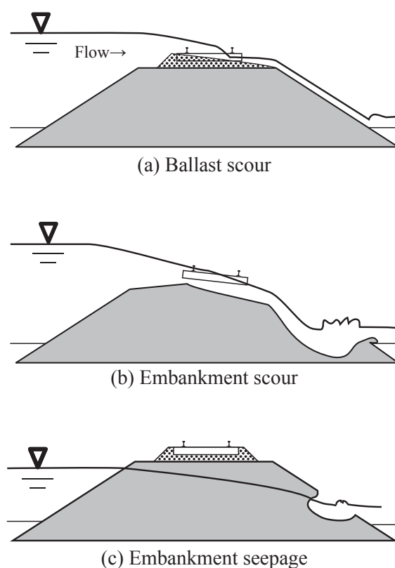
Figure 2. Railway embankment damage types.
