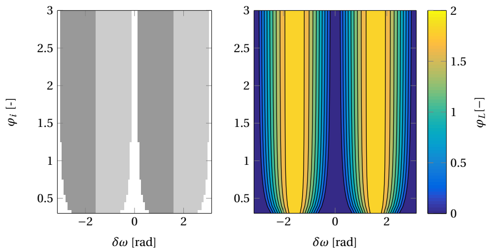
Figure 3.11: Solution to Problem 3.5 in terms of \delta\omega and \varphi_i for an Earth pointing sensor with a 9^\circ half cone angle. The graph on the left side shows whether 1. the constraint is violated at \varphi_L = 0 (white), 2. the violation occurs for \varphi_L < 0 (light-grey) or 3. the violation occurs for \varphi_L > 0 (dark-grey). The graph on the right side shows the magnitude of \varphi_L .
