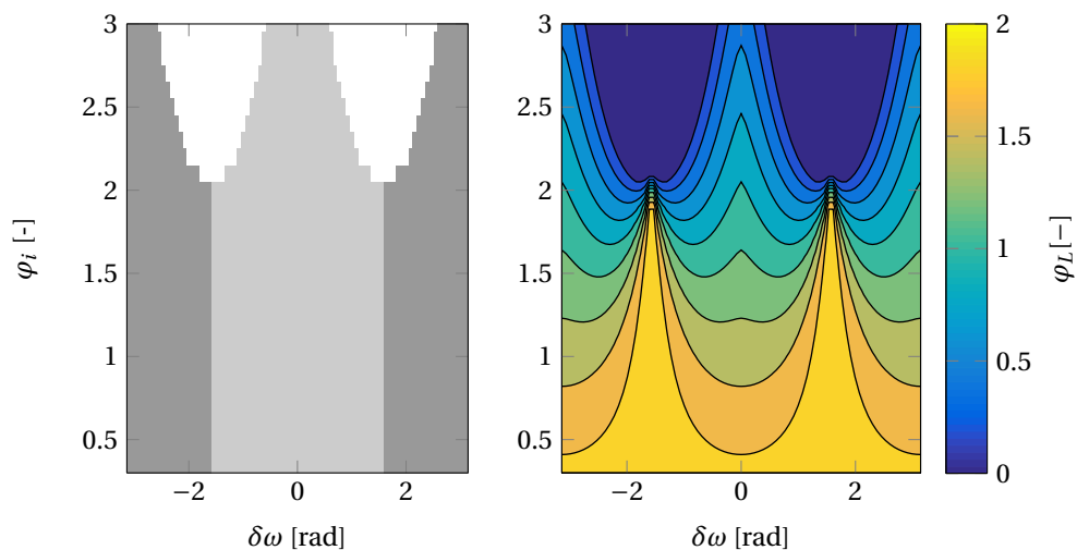
Figure 3.12: Solution to Problem 3.5 in terms of \delta\omega and \varphi_i for a North pointing star sensor with a 26^\circ half cone angle. The graph on the left side shows whether 1. the constraint is violated at \varphi_L = 0 (white), 2. the violation occurs for \varphi_L < 0 (light-grey) or 3. the violation occurs for \varphi_L > 0 (dark-grey). The graph on the right side shows the magnitude of \varphi_L .
