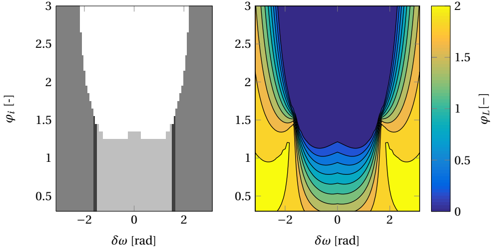
Figure 3.19: Rational Element Map for C4 - Star sensor pointing North-East. The graph on the left side shows whether 1. the constraint is violated at \phi_L = 0 (white), 2. the violation occurs for \phi_L < 0 (light-grey), 3. the violation occurs for \phi_L > 0 (dark-grey) or 4. the violation occurs for \phi_L < 0 and \phi_L > 0 (darkest-gray). The graph on the right side shows the magnitude of \phi_L .
