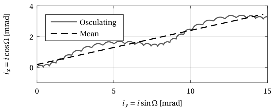
Figure 2.9: Osculating and mean variations of the inclination vector based on Kamel's synchronous satellite ephemeris
