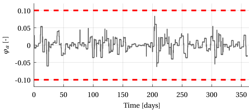
Figure 5.15: Rational relative semi-major axis, rectangular rational window, 3.5 day maneuver cycle.
