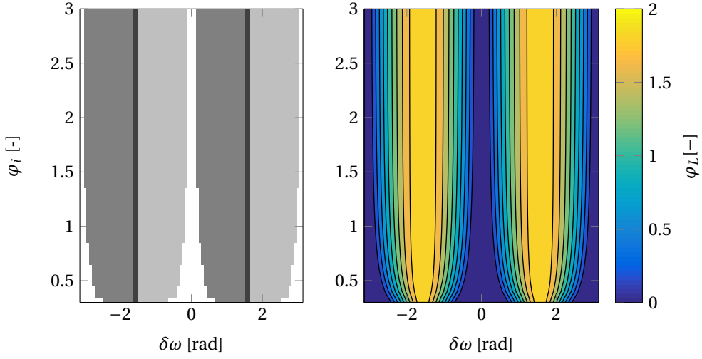
Figure 3.18: Rational Element Map for C3 - Earth pointing sensor. The graph on the left side shows whether 1. the constraint is violated at \phi_L = 0 (white), 2. the violation occurs for \phi_L < 0 (light-grey), 3. the violation occurs for \phi_L > 0 (dark-grey) or 4. the violation occurs for \phi_L < 0 and \phi_L > 0 (darkest-gray). The graph on the right side shows the magnitude of \phi_L .
