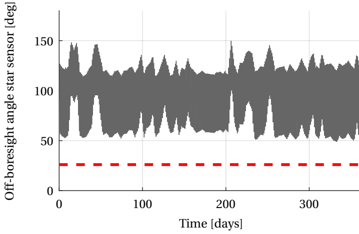
Figure 5.19: Off-boresight angle of satellite F1 with respect to a star sensor attached to the leader, rectangular rational window, 3.5 day maneuver cycle.
