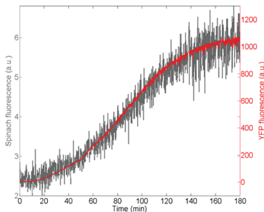
Figure 2.12: Time course of the YFP fluorescence (red trace) and corresponding cross-talk in the Spinach channel (gray trace). A concentration of 0.7 nM of the control YFP construct was used along with 20 \mu M DFHBI.
