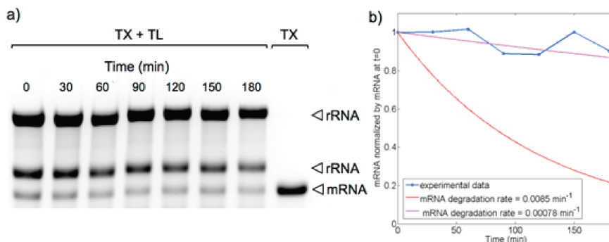
Figure 2.14: a) RNA gel showing presynthesized mRNA (from the YFP-Spinach DNA) used as a template in a translation (TL) reaction performed with the PUREflex for different time periods. The ribosomal RNA (rRNA) bands were used for normalization. The right-most lane shows the purified mRNA presynthesized in a transcription (TX)-only reaction. b) Quantification of the amount of presynthesized mRNA normalized to that of time zero and to the band intensity of the 1.5-kb rRNA at the corresponding time point. The purple and red traces correspond to the profiles of mRNA levels as found by Stögbauer et al.[16] and Niederholtmeyer et al. [18], respectively.
