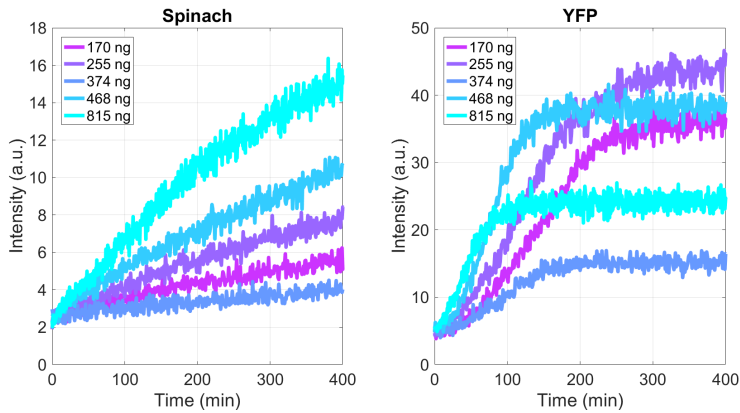
Figure 5.16: Expression kinetics of Spinach and YFP from the T7R hybrid template in the PUREfrex system.
