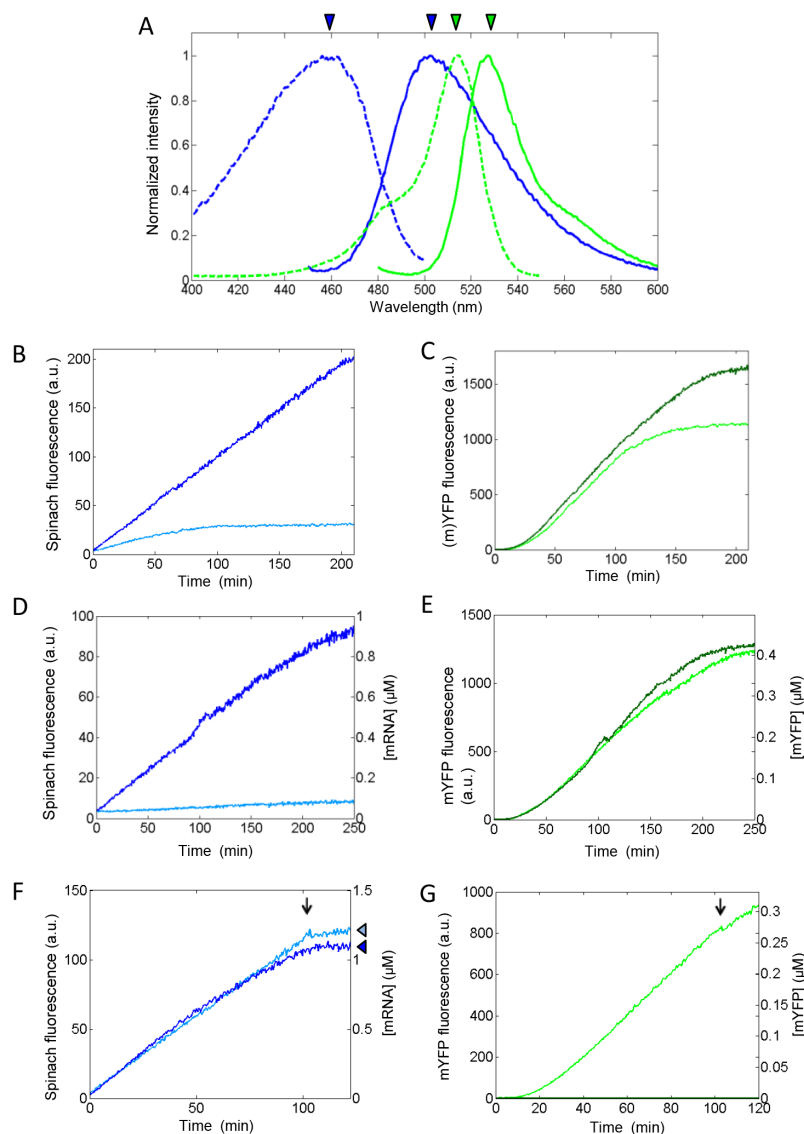
Figure 3.3: (A) Fluorescence excitation (dashed lines) and emission (solid lines) spectra of LL-Spinach (blue) and mYFP (green) measured in the PURE \Delta expressing the mYFP-LL-Spinach gene. The LL-Spinach spectra were measured in the PURE \Delta , that is devoid of ribosome, in the presence of 20 \mu M DFHBI. The mYFP spectra were collected in the PURE \Delta without DFHBI. The arrowheads depict the excitation and emission wavelengths used for kinetics measurements. (B) Fluorescence intensity profiles of Spinach produced from the mYFP-LL-Spinach (dark blue) or YFP-Spinach (light blue) construct. (C) Apparent kinetics of mYFP (dark green) and YFP (light green) synthesis monitored simultaneously as in (B). (B, C) DNA concentration for both genes was 7.4 nM. (D) Plots of LL-Spinach fluorescence versus time using the mYFP-LL-Spinach (dark blue) or mYFP (light blue) construct. (E) Apparent kinetics of mYFP produced from the mYFP-LL-Spinach (dark green) or mYFP (light green) construct and monitored simultaneously as in (D). (D, E) DNA concentration for both genes was 0.74 nM. (F) Progression of Spinach fluorescence versus time in a PURE \Delta (dark blue) or PURE \Delta (light blue) reaction starting from 11.7 nM of the mYFP-LL-Spinach DNA. The arrowheads on the right axis point to the final intensity values used for calculating the conversion factor between fluorescence a.u. and mRNA concentration. (G) Apparent kinetics of mYFP synthesis in a PURE \Delta (dark green) or PURE \Delta (light green) reaction monitored simultaneously as in (F). (F, G) The arrow at around 100 min indicates the addition of DNaseI to stop transcription. (D, F) Concentrations of mRNA were calculated using a conversion factor of 10 nM / a.u. (E, G) Concentrations of mYFP were calculated using a conversion factor of 0.33 nM / a.u.
