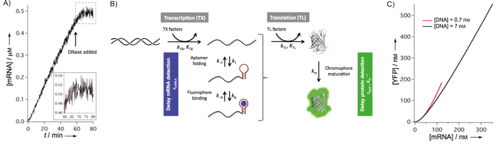
Figure 2.4: A Coarse-grained kinetic model of the transcription and translation reactions in the PURE system depends on several parameters. A) The delay time between mRNA production and its detection was quantified by measuring the residual increase of Spinach fluorescence upon YFP-spinach DNA degradation in order to ascertain a stable amount of mRNA. The red line is a monoexponential fit to the fluorescence signal shown in the dashed box, which gives an apparent maturation rate constant of 0.38 \text{ min}^{-1} \pm 0.15 \text{ min}^{-1} ( n=4 ). [\text{DNA}] = 14 \text{ nM} , [\text{DFHBI}] = 20 \text{ μM} . B) The main steps introducing a delay time between product synthesis and detection are indicated. The Spinach RNA aptamer is shown as a brown hairpin and the complexed DFHBI fluorophore as a blue circle. C) Actual concentrations of YFP versus mRNA as calculated by fitting the first 60 min of the traces in 2.2A) and B) to the reaction kinetics model presented.
