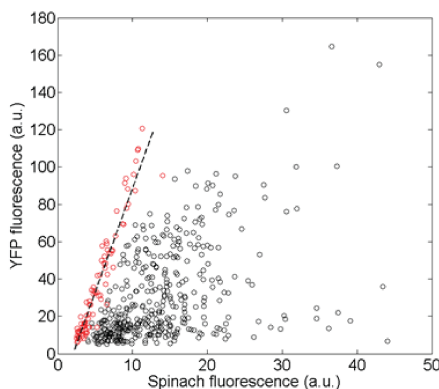
Figure 2.15: Uncorrected two-dimensional intensity plot of YFP and Spinach fluorescence inside individual liposomes. Each point represents the mean fluorescence intensities from a single vesicle. The YFP-Spinach (black circles) or the YFP (red circles) construct was used at a concentration of 30 nM. The dashed line is a linear fit to the data obtained with the YFP gene.
