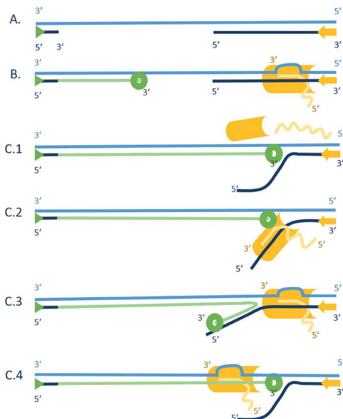
Figure 7.12: Schematic overview of possible outcomes of a head-on collision between a DNAP (green donut) and an RNAP (yellow fish). Relevant examples in literature are given in brackets. Note that outcomes C.2 and C.4 are specific to moving roadblocks, and outcomes C.1 and C.3 are essentially the same as in Figure 7.11. A) Template scheme with a fluorescently labeled primer (green triangle) that serves as a PTJ for the DNAP. The yellow arrow indicates the directionality of transcription by the RNAP starting from the promoter sequence. B) DNAP elongates the primer and RNAP starts transcription; both enzymes make use of opposite template strands. C.1) The DNAP kicks off the RNAP, leading to aborted transcription products ([25]). For moving roadblocks such as the RNAP, it is in theory also possible that the DNAP is kicked off. C.2) The DNAP displaces its non-template strand, while the RNAP remains bound to its template strand and can resume transcription ([26, 33]). C.3) The DNAP switches to the displaced strand. C.4) The DNAP passes the RNAP and the RNAP switches to the newly synthesized DNA strand ([28]).
