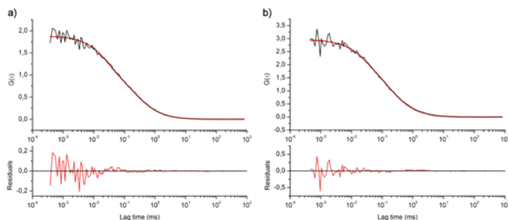
Figure 2.10: Fluorescence autocorrelation curves of a 300- or 1,800-fold diluted solution of YFP synthesized in the PUREfrex a) or PURExpress b), respectively. The fits to Eq. 2.5 (red lines) and the fit residuals (bottom graphs) are also shown.
