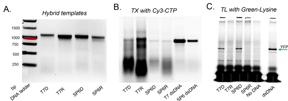
Figure 5.10: Hybrid templates are transcribed in an in vitro transcription (TX) system or transcribed and translated in an in vitro transcription-translation (TX-TL) system A.) Hybrid templates are visualized on an 1.0% agarose gel and stained with EtBr. B.) Transcription of the hybrid templates is performed in an in vitro TX kit in the presence of Cy3-CTP that is imaged with a fluorescence scanner. More non full-length RNA products are visible in the TX from hybrid lanes compared to TX from dsDNA. C.) Transcription and subsequent translation of hybrid templates is performed in the PURE ® system in the presence of a fluorescently labelled lysine amino acid (Green-Lysine). Full-length YFP peptides are produced when starting from the T7D and SP6D hybrid templates.
