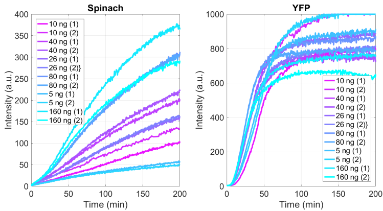
Figure 5.15: Expression kinetics of Spinach and YFP from the T7D hybrid template in the PUREfrex system.
