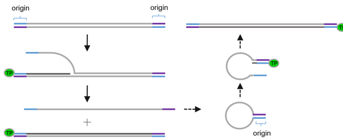
Figure 7.6: When DNA replication is only initiated at one end of the template by a TP-DNAP complex, single-strand displacement will result in the generation of ssDNAs. If the origins of replication are long (ca. 100 bp in adenoviruses) inverted terminal repeats, the ends of the ssDNA can fold upon itself creating a ds-handle and thus serve as a new initiation site. Figure is based on [21], DNAP molecule is not shown for simplicity.
