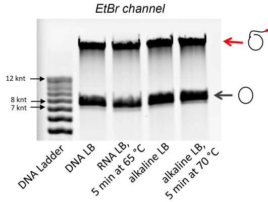
Figure 7.5: An RCA reaction performed by the phi29 DNAP is loaded on an alkaline gel with different buffers to compare the final sample quality. No difference is observed between the different treatments, which indicates that the ssDNA did not undergo cleavage under these specific conditions. Final loading buffer (LB) conditions are, DNA LB: 5% glycerol, RNA LB: 48% formamide, alkaline LB: 30 mM NaOH.
