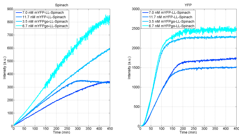
Figure 3.7: The gene optimized mYFPgo-LL-Spinach produces higher Spinach and YFP fluorescence when expressed in the PURE system compared to that with the mYFP-LL-Spinach construct (expressed at 37 °C).
