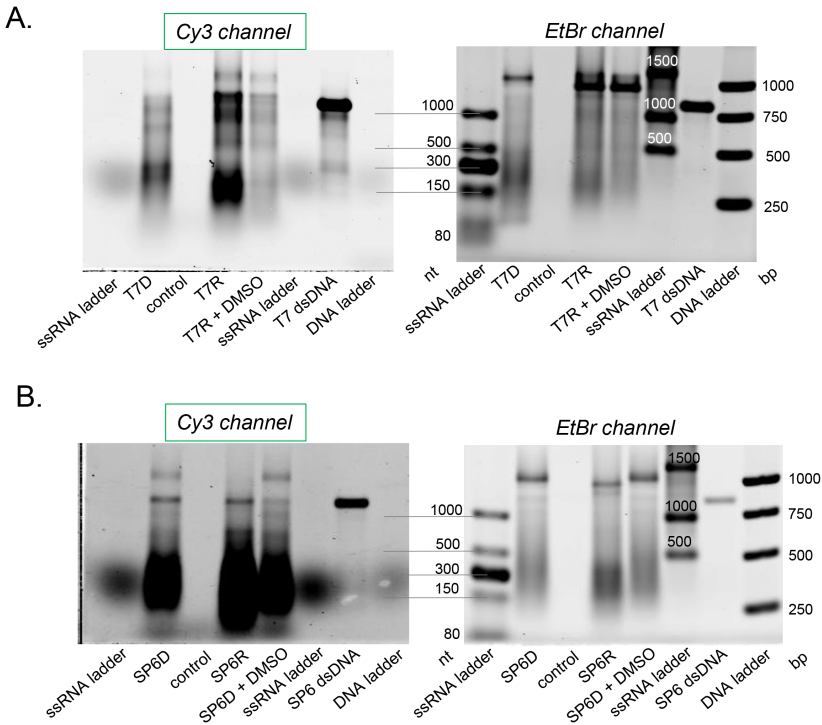
Figure 5.19: Transcription of the hybrid templates with incorporation of a fluorescently labelled Cy3-CTP imaged on RNA agarose gels for the T7 templates (A) and SP6 templates (B). Transcription from both hybrid templates generates a large amount of non-full length products (mostly between 150-500 nt), whereas this is not the case for transcription from a ds DNA template containing the same sequence. DMSO does not attenuate the formation of aborted products. The control samples were produced with the hybrid construct protocol with omission of the Accuscript enzyme. This control experiment confirms that there is no residual amount of carry over of DNA/RNA that contributes to transcription or translation reactions.
