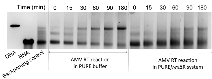
Figure 5.4: The reverse transcription reaction by the AMV RT generates two times more product after 3 h at 37 °C in the PURE buffer in comparison with the PURE system (without ribosomes). The input RNA template is purified from a transcription reaction by the SP6 RNAP on the SP6p-T7p-mYFP-LL-Spinach-polyA template. The backpriming control is a reverse transcription reaction by the AMV RT in the absence of the (dT) primer, where a small fraction (15% after 3 h compared to PURE buffer reaction) of product is formed.
