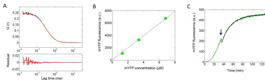
Figure 3.5: Quantification of YFP concentration and maturation time. (A) Fluorescence autocorrelation curve of a 50-fold diluted solution of mYFP synthesized in the PURExref and analyzed by FCS. The fit to Eq. 1 (red line) and the fit residual (bottom graph) are shown. (B) Quantification of PURExpress-synthesized mYFP concentration by absorbance measurements. The mYFP fluorescence intensity measured on the spectrofluorometer was plotted against the concentration determined by absorbance. The slope gives a conversion factor of 1.01 nM / a.u. (C) The maturation time of mYFP was experimentally measured by adding 3 \mu L of the translation inhibitor chloramphenicol (arrow). The residual increase in fluorescence was fitted with a monoexponential function (black curve), giving a maturation time of 20 min.
