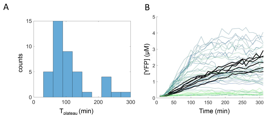
Figure 3.13: Expression time of the YFP varies between liposomes. A) Histogram (counts) of the plateau times T_{plateau} of the YFP kinetic curves shown in Figure 3.11. Plateau times are determined as in Section 3.5. Plateau times higher than 300 min are left out of this histogram (see Figure 3.16 as they do not represent an actual experimentally measured plateau time. B) Some of the kinetic curves that do not reach a plateau during the time of measurement are highlighted in black.
