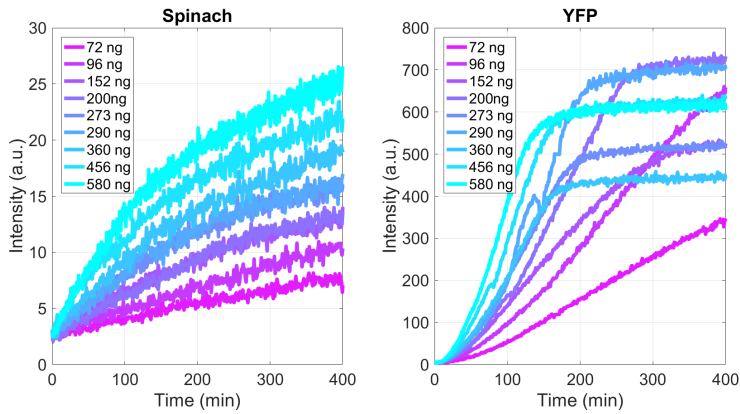
Figure 5.14: Expression kinetics of Spinach and YFP from the T7 dsDNA template in the PUREfrex system.
