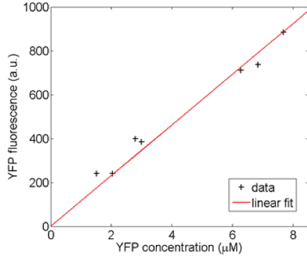
Figure 2.11: Calibration of YFP concentration generated with the PURExpress. Data from three independent experiments are reported.
