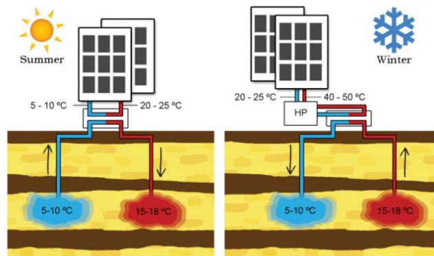
Figure 1: Use of soil energy by ATES; © KWR, Martin Bloemendal
