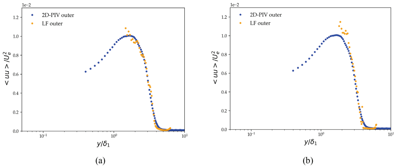
Fig. 5 Reynolds stress profile \langle uu \rangle of LF-PIV at different z positions comparing with 2D-PIV. The figure (a) is z = -1.525\text{ mm} and (b) is z = -0.696\text{ mm} , relative to the center of the camera's focal plane ( z = 0\text{ mm} ).
