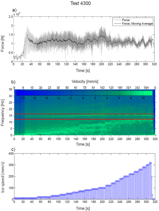
Fig. 3. (a) Time history of the force, (b) frequency variation with respect to time, and (c) ice speed range for Test 4300 (from Nord et al. (2015)).
