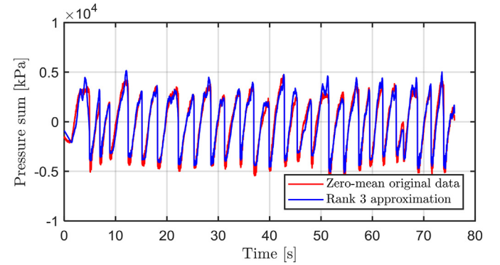
Fig. 12. Example time history of the sum of pressures for the zero-mean original data (red) and rank-3 approximation (blue) at 5 \text{ mm s}^{-1} ice speed obtained using IRPCA algorithm. (For interpretation of the references to colour in this figure legend, the reader is referred to the web version of this article.)
