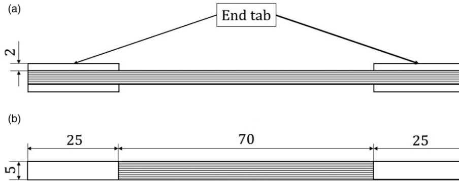
Figure 4. Geometry of tensile specimens, (a) side view, (b) top view, (dimensions in mm).
