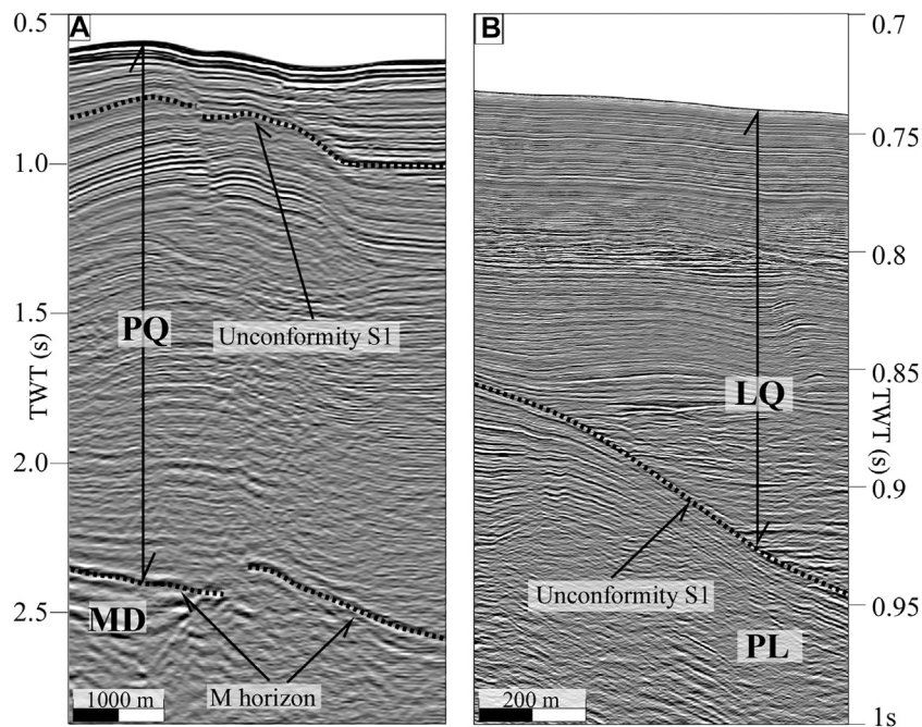
FIGURE 4 | (A) Seismostratigraphic units (MD and PQ) recognised on the high-penetration seismic profile "Line Sister—12". (B) Seismostratigraphic subunits (PL and LQ) recognised on the HR seismic profile "Line—04." See Figure 5A for location.
