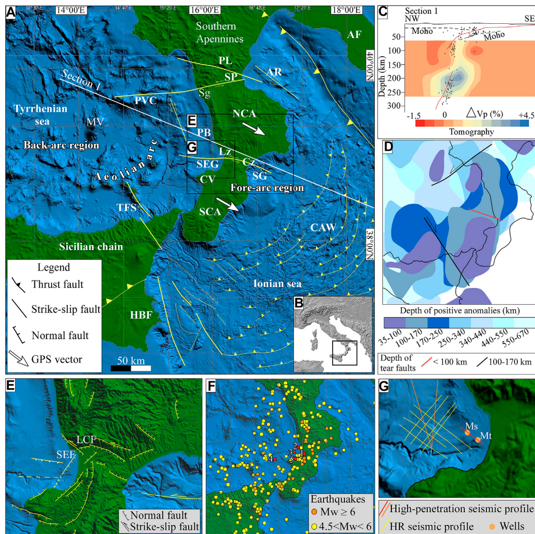
FIGURE 1 | (A) Schematic tectonic map of the Tyrrhenian-Ionian subduction system. AF, Apulian foreland; AR, Amendolara ridge; CAW, Calabrian accretionary wedge; CV, Capo Vaticano; Cz, Cosenza; HBF, Hyblean foreland; Lz, Lamezia; MV, Marsili volcano; NCA, northern Calabrian Arc; PB, Paola basin; PL, Pollino; PVC, Palinuro volcano complex; SCA, southern Calabrian Arc; SEG, Sant'Eufemia Gulf; Sg, Sangineto; SG, Squillace Gulf; SP, Sibari Plain; TFS, Tindari fault system. (B) Location of the area shown in panel a. (C) Section across the slab (modified from Maesano et al., 2017). Redline is the position of the subduction interface. Black dots are the earthquakes collected in 10-km wide buffers around the section trace. The dashed black line is the position of the Moho from Scrocca et al., 2003. Tomographic data are from Neri et al., 2009. (D) Upper mantle structure based on positive P wave seismic anomalies (modified from Rosenbaum et al., 2008). The coloured areas represent positive anomalies at different depth ranges. Rosenbaum et al., 2008 interpreted these areas as remnant subducting slabs, separated by tear faults (black and red lines). (E) Schematic tectonic map of the central Calabrian Arc (modified from Monaco and Tortorici, 2000; Brutto et al., 2016) and offshore (modified from Loreto et al., 2013; Del Ben et al., 2008). LCF, Lamezia-Catanzaro Fault; SEF, Sant'Eufemia Fault. (F) Distribution of instrumental earthquakes recorded since 1985 up-to-date, from INGV Seismic Bulletin (ISide Working Group, 2007; http://iside.rm.ingv.it ). Red squares indicate the 1905 epicentral location proposed by (1) Rizzo, (1906), (2) Riuscetti and Schick, (1975), (3) Camassi et al. (1997), (4) Michelini et al. (2006), (5) Guidoboni et al. (2007). (G) Grid of high-penetration and high-resolution (HR) seismic profiles used for this study. Ms, Marisa well; Mr, Marta well.
