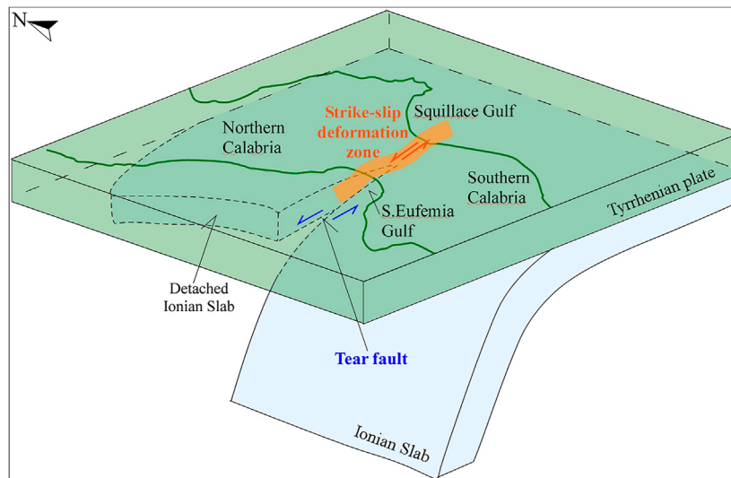
FIGURE 10 | Geodynamic sketch of the Tyrrhenian-Ionian subduction system illustrating the strike-slip deformation zone extending from Sant'Eufemia Gulf to Squillace Gulf formed above the tear fault inferred between two segments of the Ionian slab.
