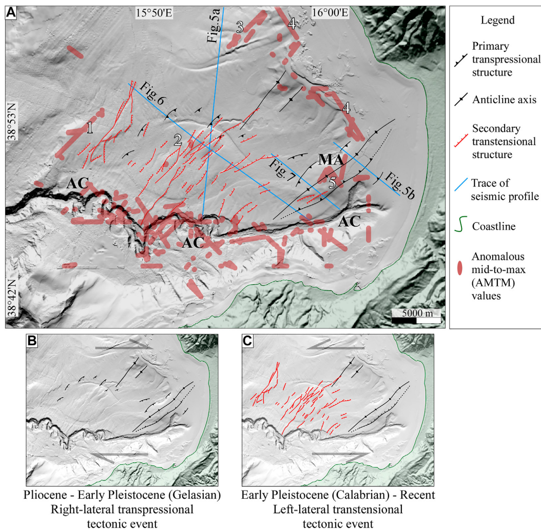
FIGURE 8 | (A) Structural map of the Sant'Eufemia Gulf. Red dots are the AMTM values localised at the intersection points of their related swath profiles. MA, Maida Ridge; AC, Angitola Canyon; 1, 2, 3, 4, and 5, sectors with alignments of AMTM values. (B and C) Schematic structural maps showing the active structures during the Pliocene—Early Pleistocene (Gelasian) and Early Pleistocene (Calabrian)—Recent tectonic events that affected the Sant'Eufemia Gulf. The activity of the structures is inferred from the analysis of seismic profiles and swath profiles (AMTM values).
