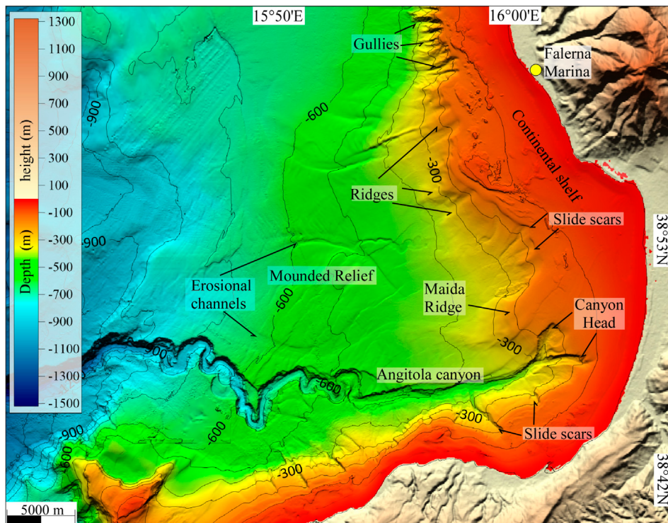
FIGURE 3 | Morphobathymetric map of the Sant'Eufemia Gulf.
