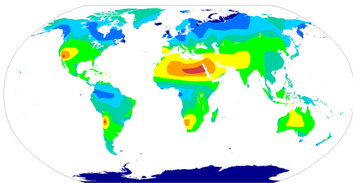
FIGURE 30: ANNUAL SUNSHINE HOURS MAP OF THE WORLD
