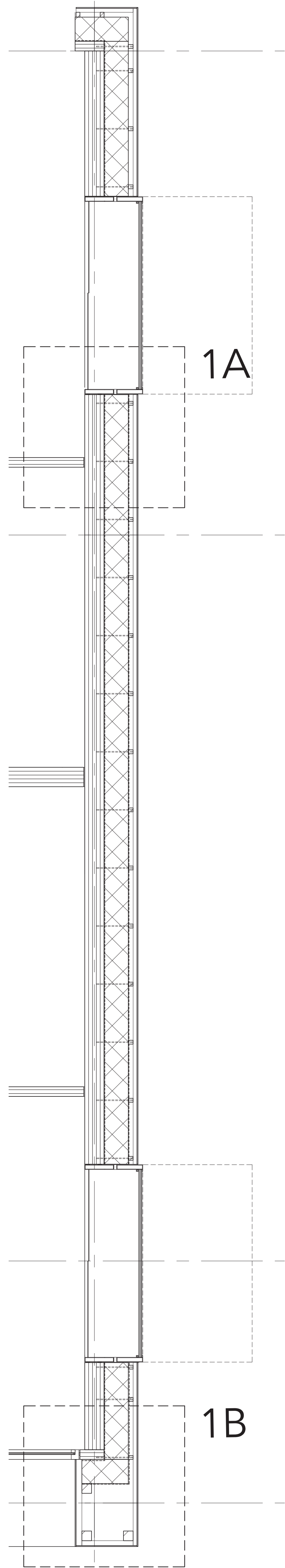
FACADE FRAGMENT (H/V) 1:20
