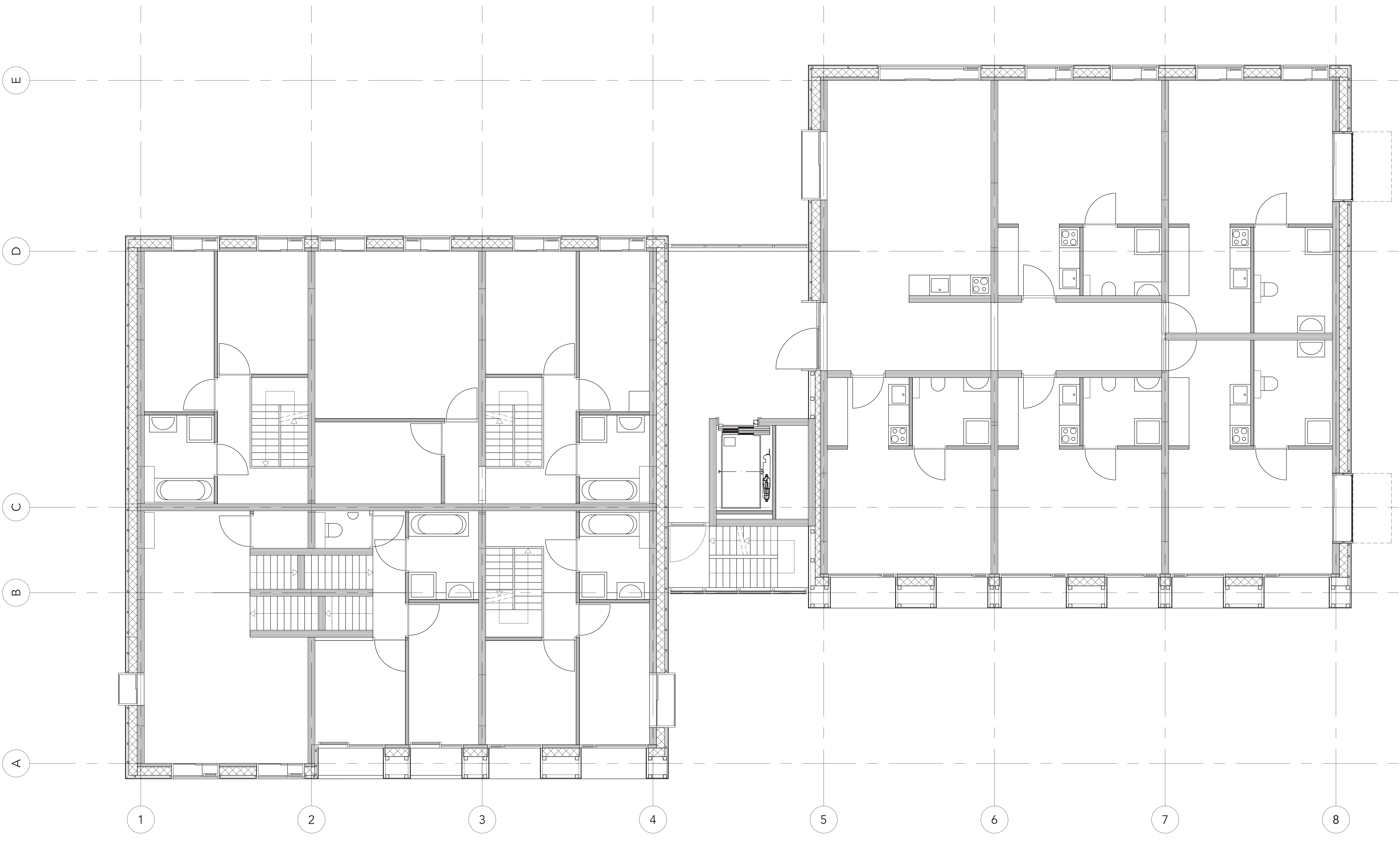
BT PLAN 1:50
