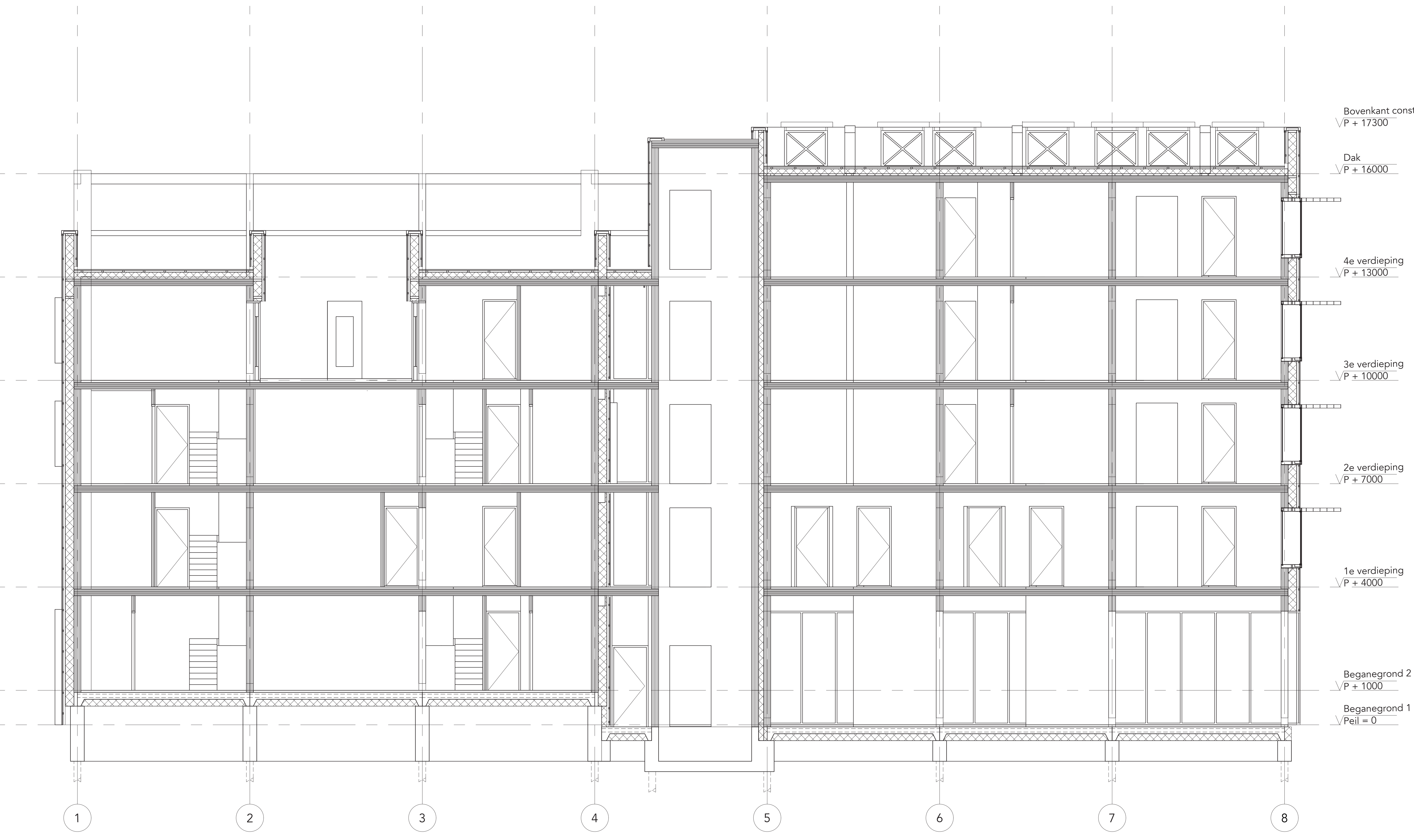
BT SECTION 1:50
