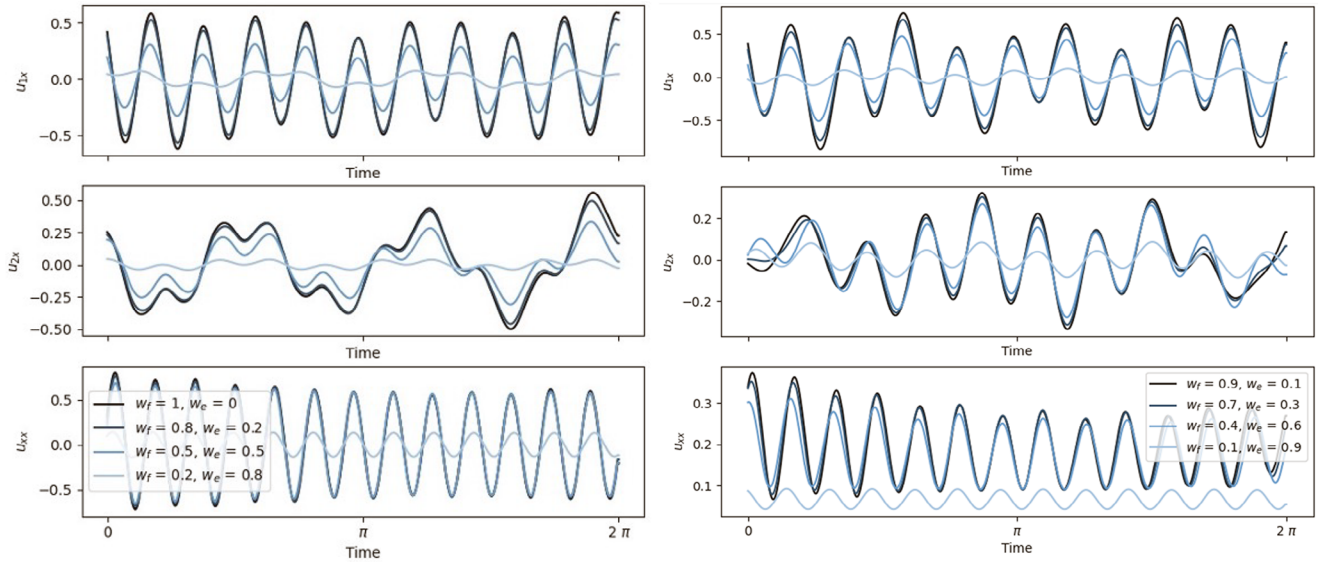
Figure 3. Example control pulses generated by the EO-GRAPe algorithm for different weight settings. Parameters: U_T = \text{RAND} , \hat{H}_D = \hat{H}_D^2 , \hat{\sigma}_k \in \{\hat{\sigma}_x^1, \hat{\sigma}_x^2, \hat{\sigma}_x^1\hat{\sigma}_x^2\} , T_1 = \infty , T_2 = \infty , w_f = [1, 0.1] , w_e = [0, 0.9] , N = 500 , N_G = 500 .
