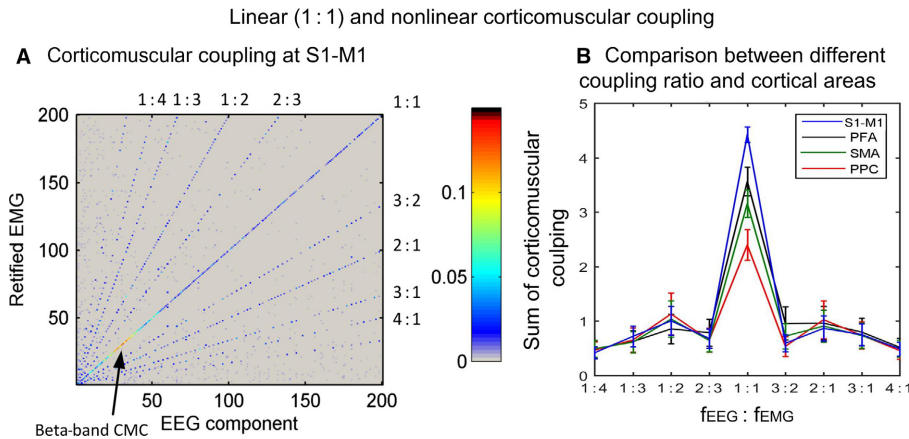
FIG. 3. Linear and nonlinear corticomuscular coupling in healthy participants during an isotonic wrist flexion task. (A) Both linear (1 : 1) and nonlinear ( n : m, n \neq m ) coupling are detected. Linear coupling shows a peak in the beta-band. (B) Comparison of corticomuscular coupling between different coupling ratio and cortical areas. The linear coupling significantly reduced from the motor-related cortical areas to sensory-related areas, while no significant differences between different cortical areas are detected for nonlinear coupling. Due to the limited spatial resolution of EEG, the activities from S1 and M1 cannot be separated. The figure is reproduced, with permission, from Yang et al. (2016a) published in Frontiers in Computational Neuroscience .
