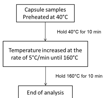
Figure 2. Thermogravimetric analysis (TGA) temperature control program.
