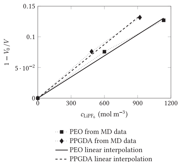
Fig. 3. Partial molar volume of \text{LiPF}_6 in PEO and PPGDA solid electrolytes.
