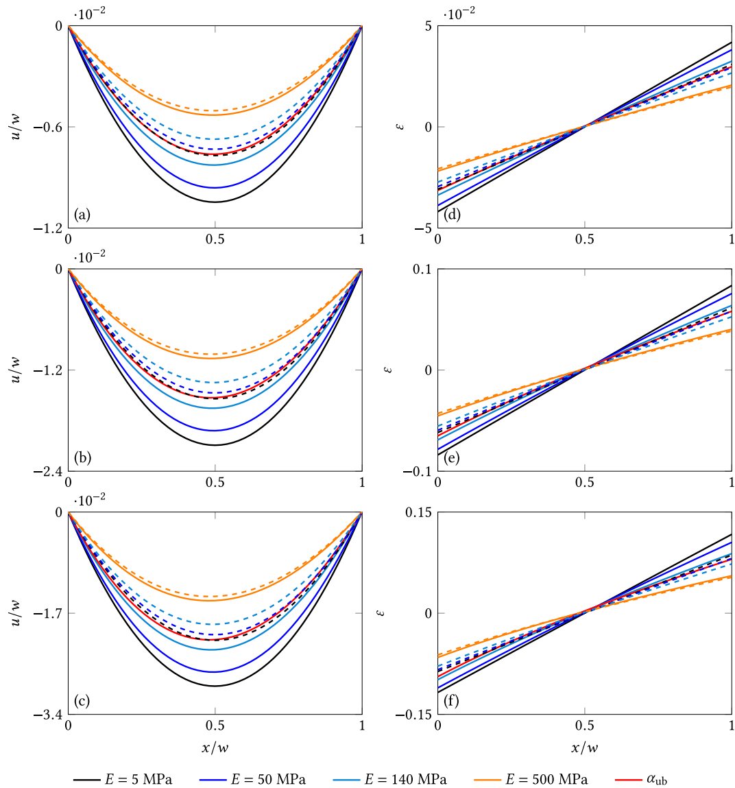
Fig. 5. Steady state profiles of the displacement (a–c) and deformation (d–f) distributions within the solid polymer electrolyte. Plots refer to three different width of the SPE: (a,d) w = 5 \mu\text{m} ; (b,e) w = 10 \mu\text{m} ; (c,f) w = 14 \mu\text{m} . The x -coordinate along the width of the SPE and the displacement are normalized by the width w itself. Continuous lines refer to \Omega = 1.5 \times 10^{-4} \text{ m}^3 \text{ mol}^{-1} , dashed lines refer to \Omega = 1.1 \times 10^{-4} \text{ m}^3 \text{ mol}^{-1} .
