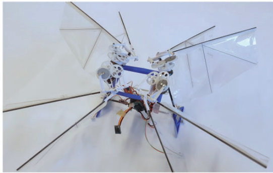
Figure 10. Photo of the final quad-thopter prototype.
