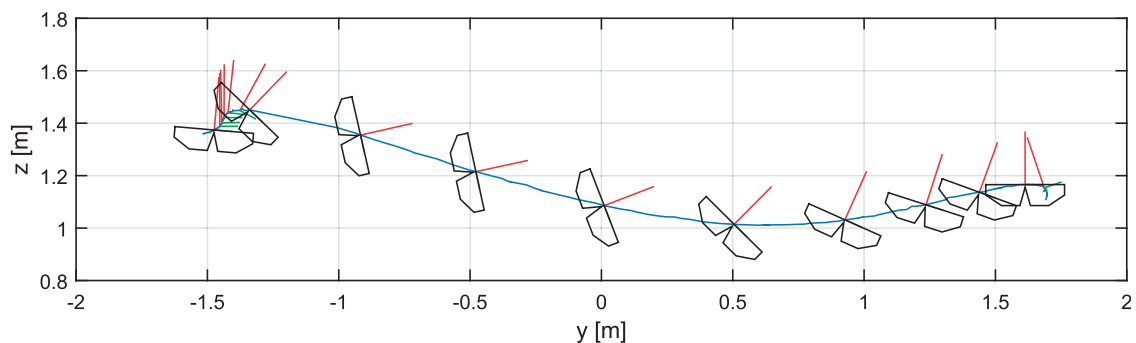
Figure 16. A 3-m lateral command where speeds of 3.5 m/s and angles of 80^\circ roll are reached.
