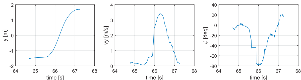
Figure 17. Position, speed, and attitude captured by an external optitrack motion tracking system during a 3-m lateral step command.
