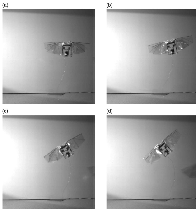
Figure 11. High-speed camera recordings at 66.6 ms interval show a step in attitude from hover to a steady 40^\circ of roll being executed in less than 266 ms or less than four wing beats at 15 Hz.
