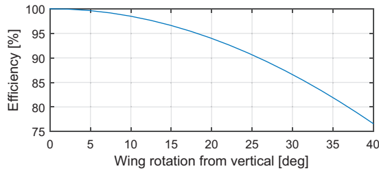
Figure 9. Efficiency in function of thrust rotation.
