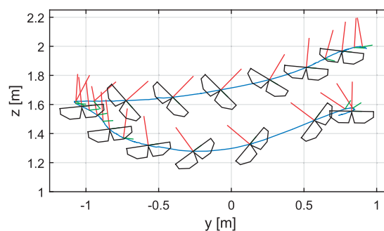
Figure 12. Indoor test flight recorded by Optitrack. The quad-thopter starts at the bottom right and makes a 2 m step to the left and then back to the right in under 3 s. Note that the vehicle does not need negative roll during the slow down.
