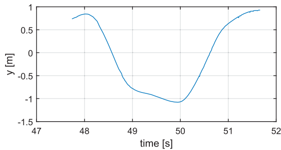
Figure 13. Lateral position change in function of time during the lateral step shown in Figure 12.
