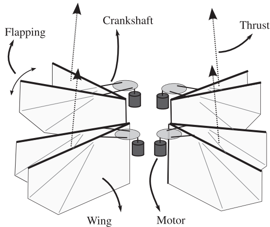
Figure 4. Quad-thopter. Four pairs of flapping wings are arranged in an X-configuration with a small angle between thrust vectors to allow control of the yaw axis.
