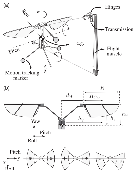
Figure 3. MAV designs that use their main actuators also for control: (a) piezo actuators 14 and (b) brushed DCs. 19
