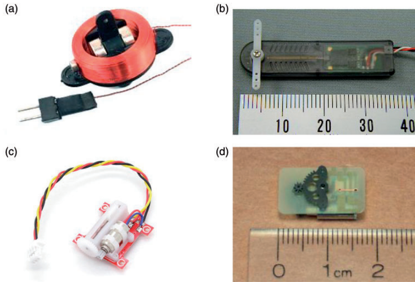
Figure 2. Overview of actuator types for lightweight flapping wing MAVs: (a) magnetic servos, (b) shape memory alloy servos, and (c, d) servos with brushed DCs (images from www.microflight.com , www.servoshop.co.uk , www.hobbyking.com , www.microflierra.io.com ).
