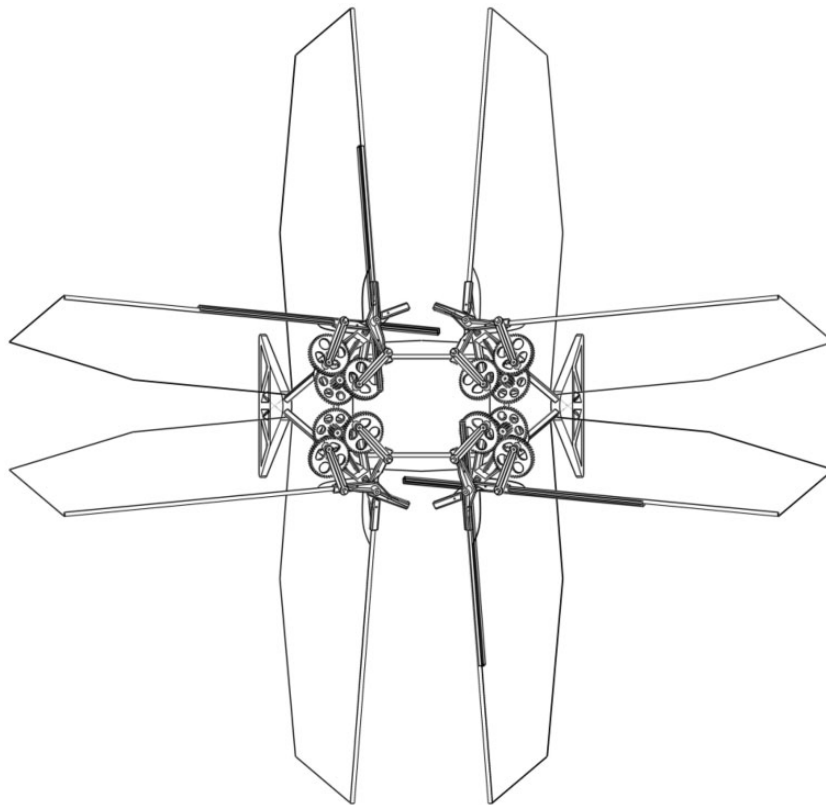
Figure 5. Quad-thopter final prototype – top view. When thrust vectors are non-parallel, two opposing pairs of wings can create a yaw moment. The maximal dimension is 28 cm from tip to tip and the weight is 37.9 g with a 205 mAh battery.
