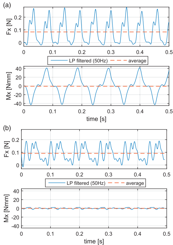
Figure 6. Thrust force and moment around principal body axis (data include also inertial effects): (a) single wing flapping with 90^\circ amplitude and (b) double-wing flapping in antiphase with 40^\circ amplitude. The reaction torque on the body is significantly reduced when using the double-wing setup while generating a similar amount of thrust as the single wing.
