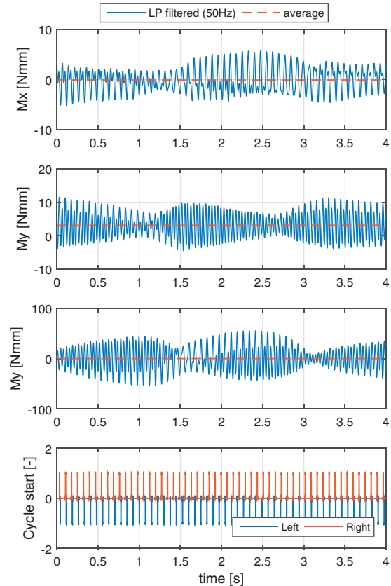
Figure 7. Two double-wing experiment: A beat phenomenon can be observed in the moment data when a difference in flapping frequencies of left and right double-wings is present. The cycle start is detected by a hall effect sensor and a magnet attached to the flapping mechanism. The residual vibration is especially strong around the roll (z) axis.
