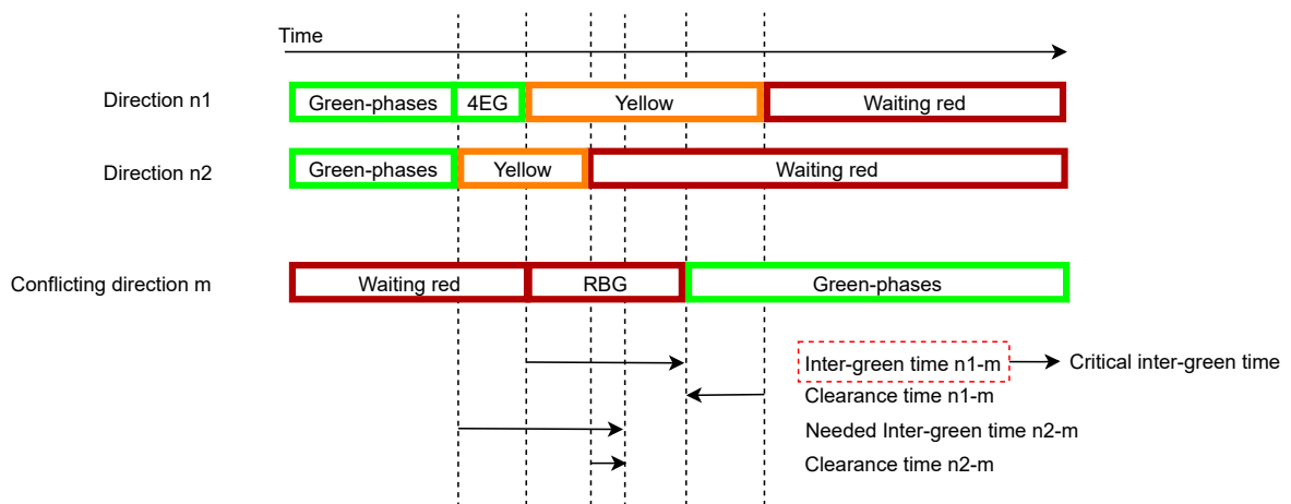
Figure 3.10: The critical inter-green time
