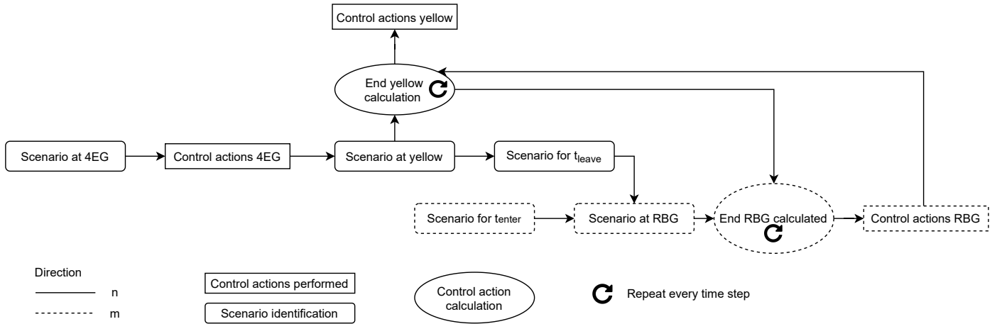
Figure 1: The connection between (sub-)phases of conflicting directions. This shows that scenario and the control actions of the same direction but also of conflicting directions are influenced by each other. The RBG phase of direction m can only be calculated when the end of yellow of direction n can be calculated.
