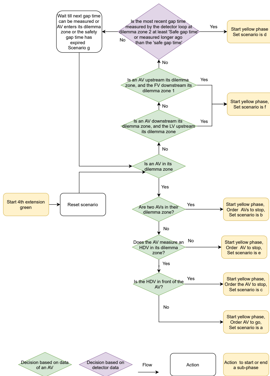
Figure 9: The flow of the controller in the 4EG phase
