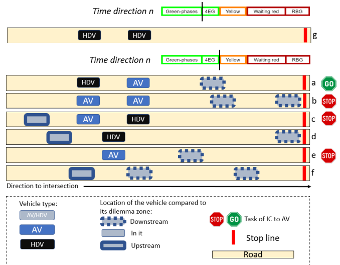
Figure 3: Possible scenarios at the start of the 4EG phase and what actions to take
