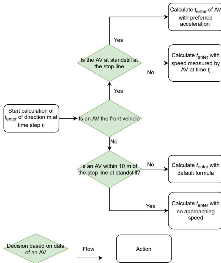
Figure 3.13: Decisions to identify scenarios for t_{enter} and its control actions
