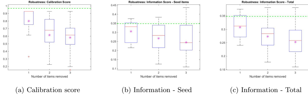
Figure 5: Robustness box-plots concerning (a) the calibration score, (b) the information score over the seed items and (c) the information score over all the queried variables of the DM_{global} , when excluding up to three seed items at a time.
