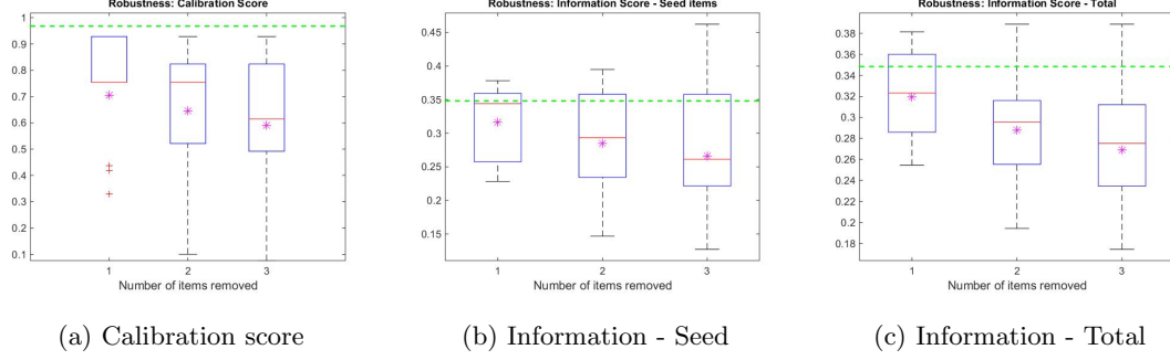
Figure 4: Robustness box-plots concerning (a) the calibration score, (b) the information score over the seed items and (c) the information score over all the queried variables of the DM_{item} , when excluding up to three seed items at a time.
