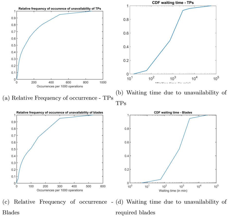
Figure 6: Obtained distributions concerning the relative frequency of delays due to unavailability of the required TPs (a), blades (c) and the waiting time due to unavailability of the required TPs (b), blades (d).
