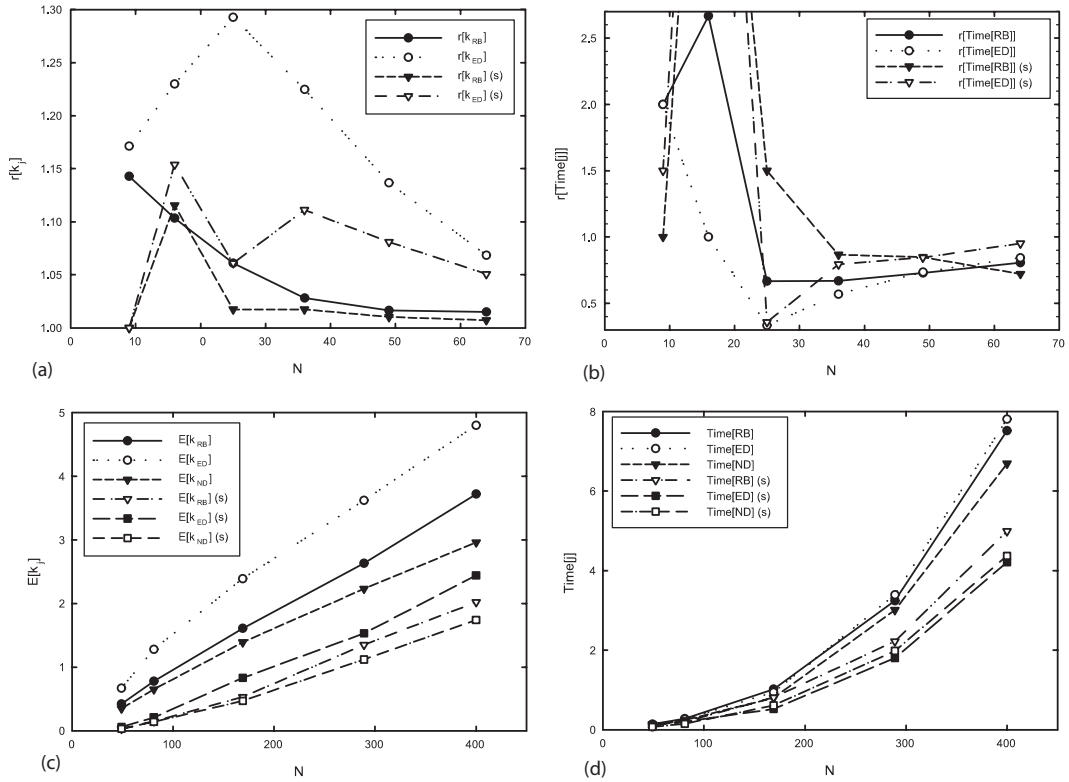
Fig. 1. The results (s denotes strict constraints) for the class of lattices as a function of the number of nodes N ( m = 2 ). The ratio of k (a) and the ratio of time (b) for \rho = -1 . The expected queue size E[k] (c) and the expected time Time[j] in seconds (d) for \rho = 0 .
