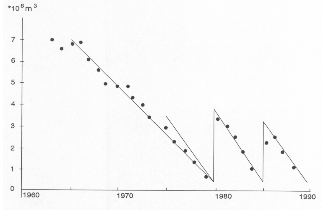
Figure 3: Coastal volumes at Texel, km 25-31, from RAKHORST [1989]
