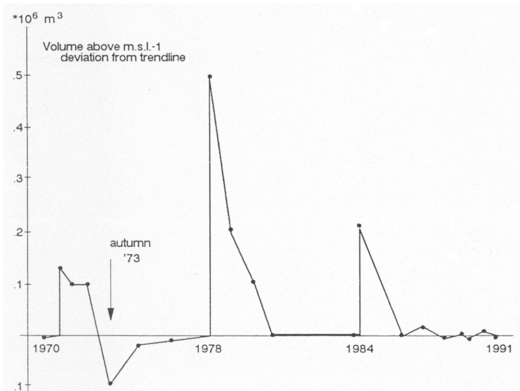
Figure 5: Volume differences from linear trend (Sylt), from FÜRHBÖTER [1991]
