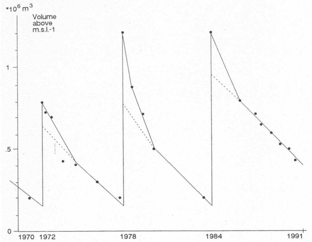
Figure 4: Coastal volumes at Sylt (Westerland), from FÜRHBÖTER [1991]
