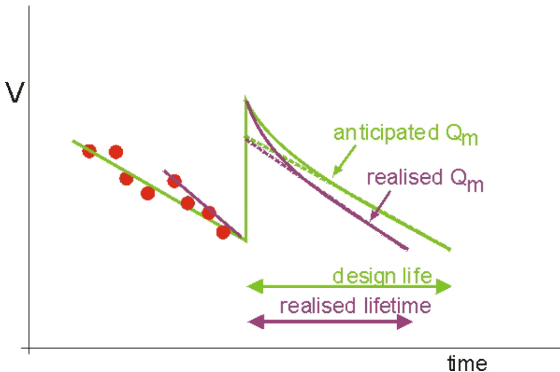
Figure 6: Design error type 1, Q_m was not determined correctly
