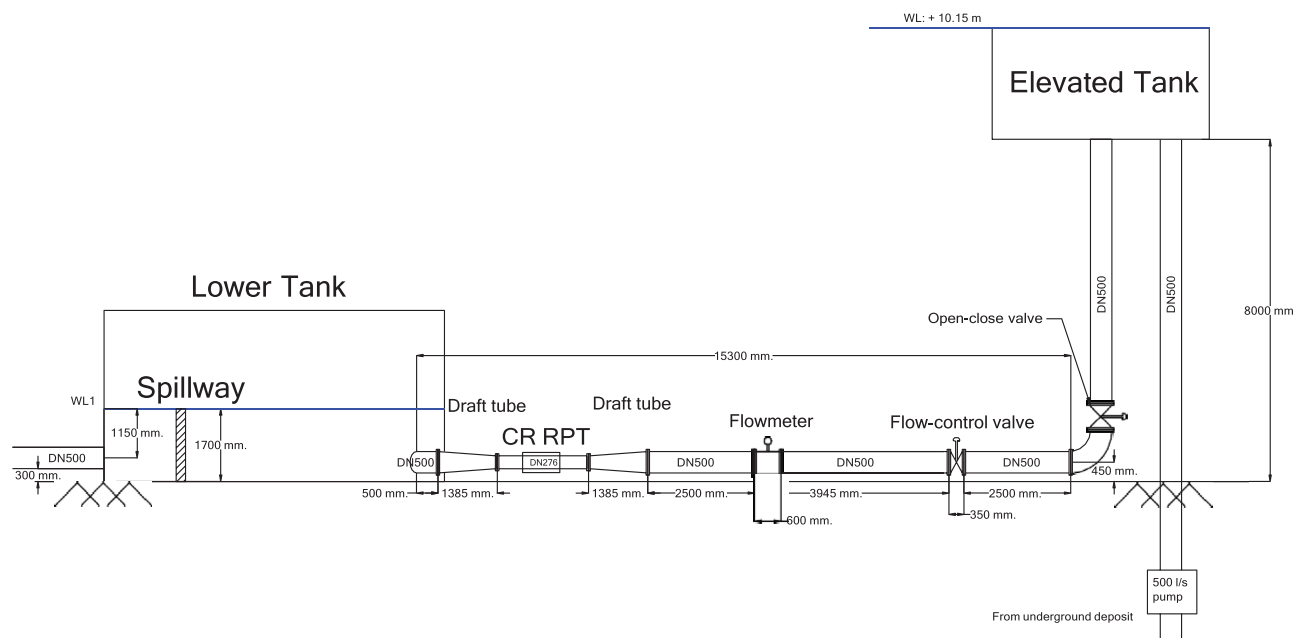
FIGURE 5 Pipe 1 design
