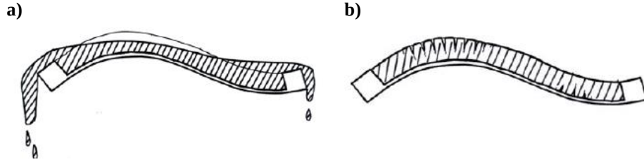
Fig. 2. Two boundary conditions for the mould deformation a) maintaining stability through an adequate yield strength and b) prevention of significant cracking through strain capacity [1].
