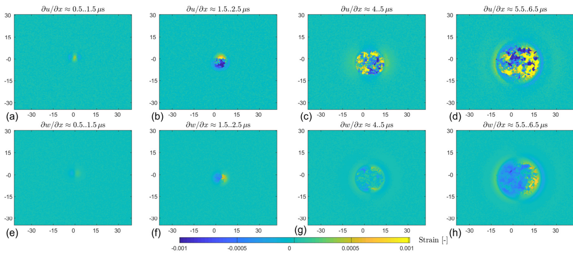
Figure 4. In- and out-of-plane surface strain maps ( \partial u/\partial x and \partial w/\partial x ) of 4 mm aluminium plates (6082-T6) at the time from 0 to 5.5..6.5 \mu s after the impact (axes units mm).
