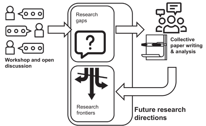
Fig. 3. Paper methodology.
