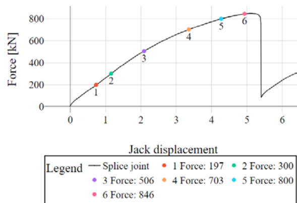
Figure 7. Load-displacement static after fatigue with indication load levels of strain reading
