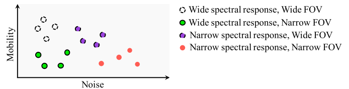
Fig. 3. Trade-offs of the receiver spectral response S_{RX} and the FOV.
