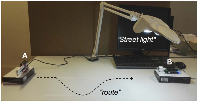
Fig. 18. Application test: route of the mobile nodes and environment setup. Two different types of LEDs are used in the experiments to support different communication distance: (i) the White LED with a FOV of 160^\circ (cf. Fig. 13), and (ii) a 3W PinYuanLighting LED with a FOV of 60^\circ .
