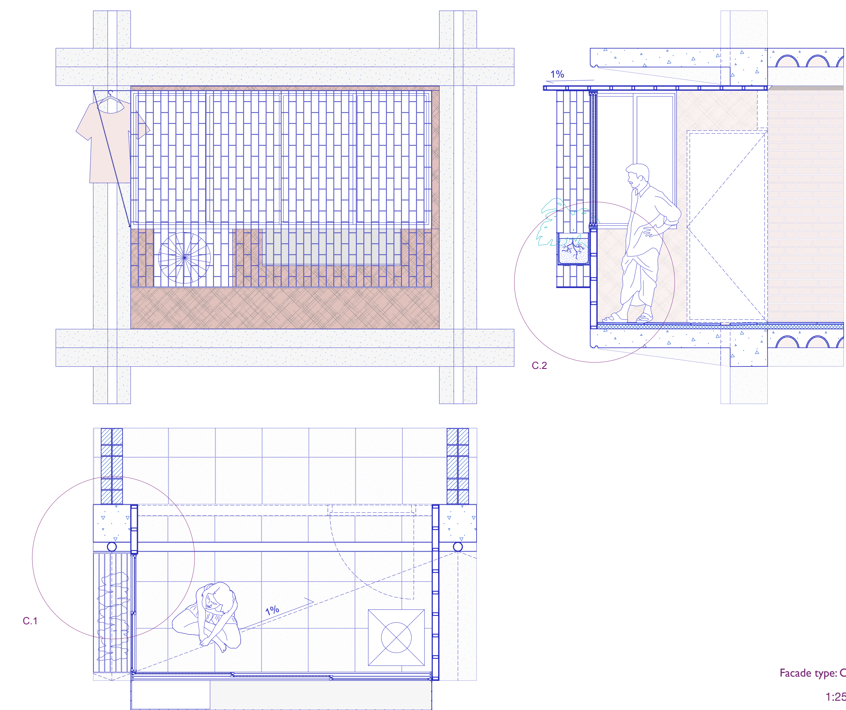
Facade type: D 1:25
