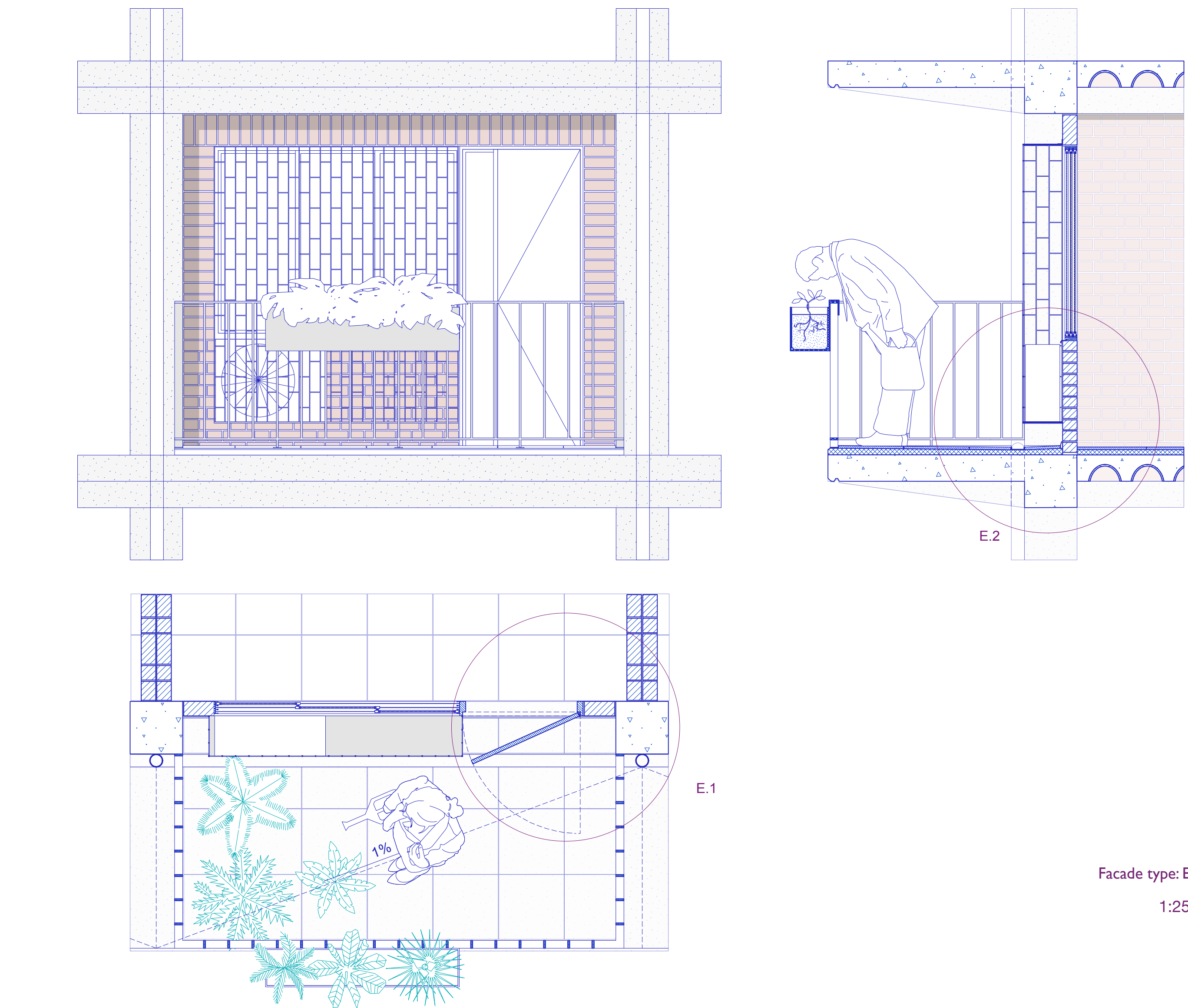
Facade type: F 1:25
