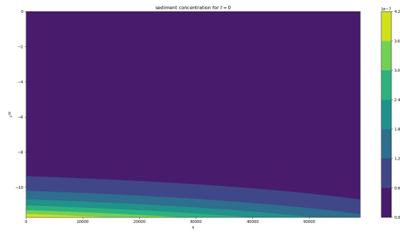
Figure 3.5: Sediment concentration at t = 0 in base system
