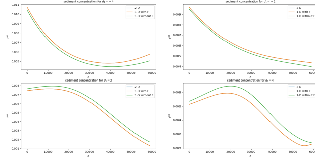
Figure 3.35: Sediment concentration with non-constant seabeds in 1D and 2D models
