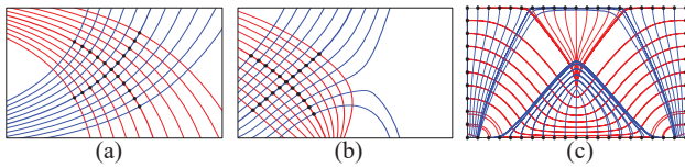
Figure 2: (a, b) Minor Principal Stress Lines (PSLs) (blue) are seeded at equally spaced seed points (●) along the initial PSL (bold orange). Additional major PSLs (orange) are then seeded along one of the minor PSLs (bold blue). (a) The resulting grid cells do not represent the local stress ratio. (b) The domain is incompletely covered. (c) PSLs concentrate despite uniform seeding density along the domain boundaries.
