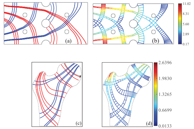
Figure 11: Perforated plate (top) and 2D femur slice (bottom). Optimized support trajectories (left), and conforming lattice with von Mises stress encoded along principal directions (right). In the femur stress field, PSLs cannot reach the boundary in the right upper region, because of the two degenerate points (black circles).
