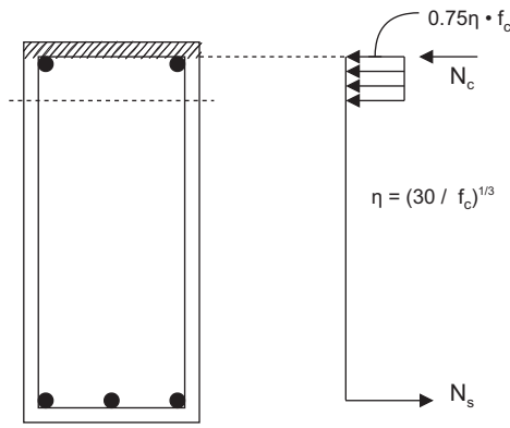
FIGURE 4 Assessment of bending capacity of a cross-section with corroded reinforcement.
