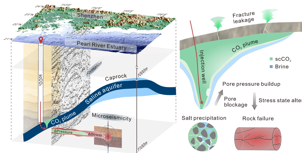
Figure 1. Schematic illustration of possible processes induced by \text{scCO}_2 injection in the Pearl River Estuary, including salt precipitation, pore blockage, pressure buildup, rock failure, and associated microseismicity.
