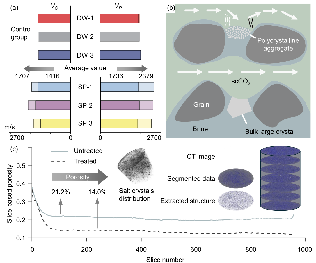
Figure 2. Effects of salt precipitation on wave velocity and pore structure in sandstone samples. (a) P- and S-wave velocity variations before and after experiments for the control (UT) and SP groups, showing significant increases in the SP group. (b) Schematic illustration showing two types of salt crystal morphologies, bulk large crystals and polycrystalline aggregates. White arrows indicate the scCO_2 flow direction. (c) CT-based analysis showing the CT processing workflow, the distribution of salt crystals concentrated within approximately 1.5 cm from the injection inlet after salt precipitation, and porosity reduction in this region, representing the general trend observed in most samples and consistent with prior studies.
