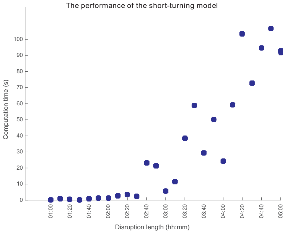
Fig. 20. The computation time of the short-turning model.
