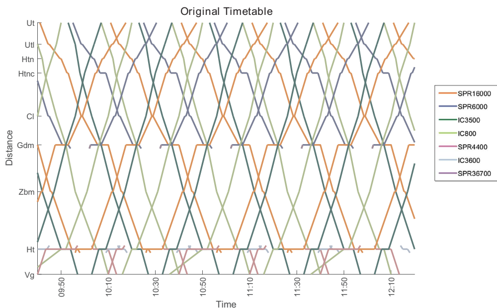
Fig. 10. The time-distance diagram of the original timetable.
