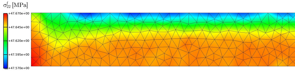
Figure 12: Spatial distribution of transverse tension strength in the macro specimen after ageing.
