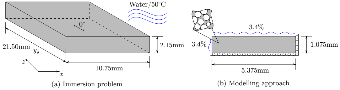
Figure 8: Modelling hygrothermal ageing in a unidirectional composite short-beam.
