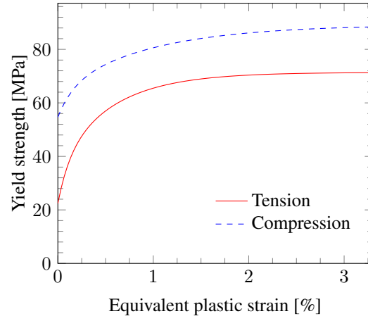
Figure 3: Input hardening data for the epoxy model.
