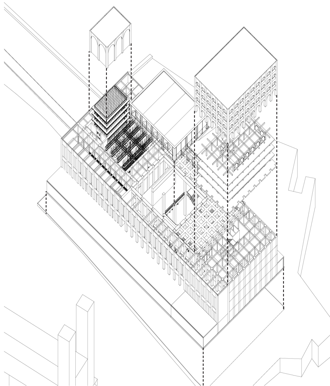
Overall Axonometric Drawing
