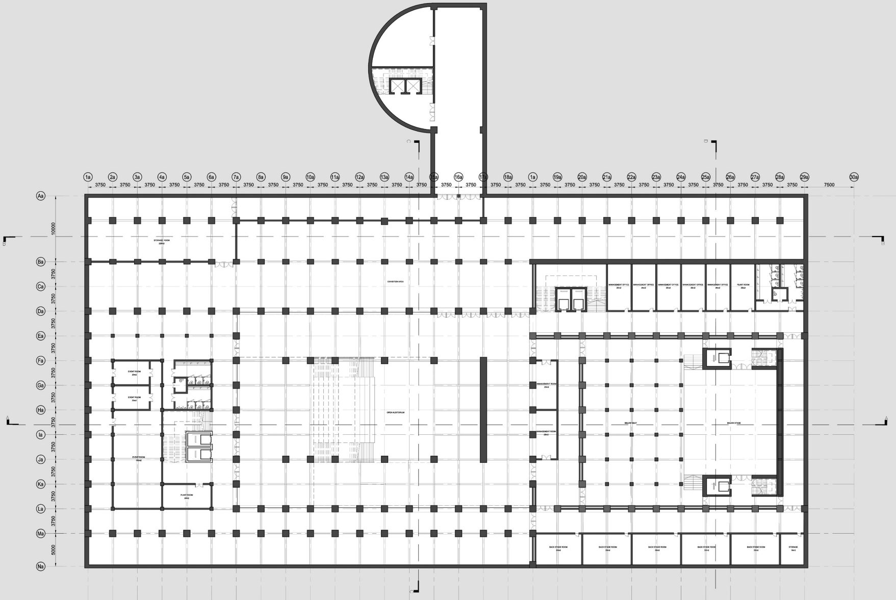
floorplan of event space level (level -4)
