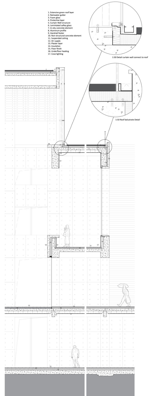
Facade Details
