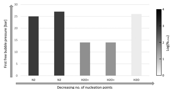
FIG. 6. Pressure where the first free bubble occurs for \text{CO}_2 saturated water starting at 30 bar. Initial fluid used to pressurize the cell is given below each bar. Grayscale indicates the peak of the number of bubbles that is formed during the experiment.
