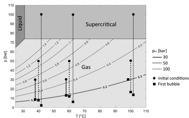
FIG. 4. Iso-solubility contours for CO 2 dissolved in brine (mol/l) as a function of temperature and pressure superimposed on the CO 2 phase diagram. The 0.2 mol/l contour is shown as a thicker line, because this is the concentration that was used in these experiments. The vertical lines in the figure indicate the depressurization path for the experiments conducted in this study.
