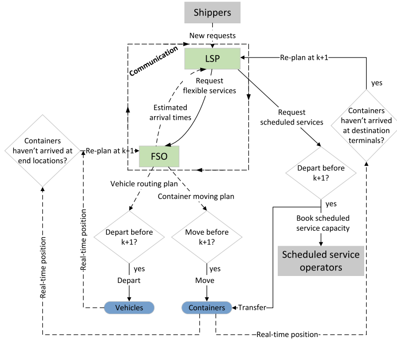
Fig. 5. Communications and actions between the LSP and the FSO under the synchromodal co-planning paradigm.
