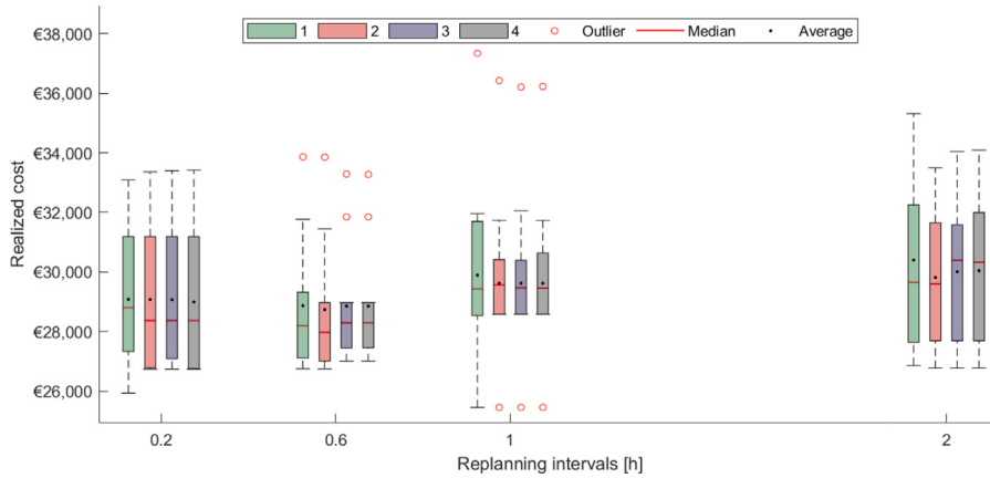
Fig. 11. The combined impact of replanning interval [h] and number of communication rounds on the performance of co-planning in terms of realized cost.
