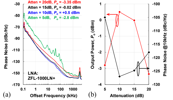
Figure 7: (a) Overall phase noise variations and (b) output power and phase noise at 10-kHz offset with respect to different attenuation.
