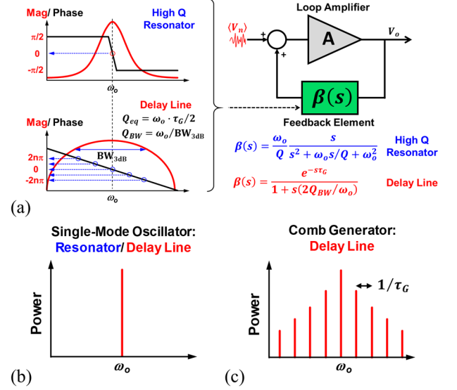
Figure 1: (a) LTI model representation for general oscillators employing a high-Q resonator or a delay line as the frequency selection element. (b) Output spectrum for a single-mode oscillator, and (c) comb-generator.
