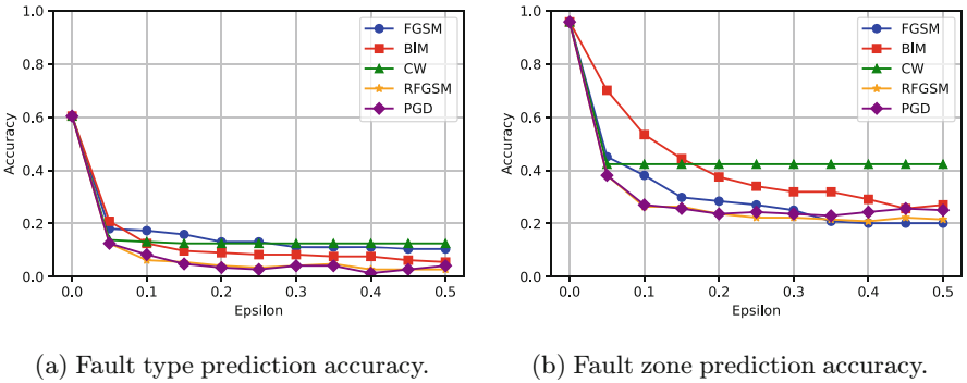
Fig. 4. Model’s accuracy at varying epsilon values on the white-box attacks.
