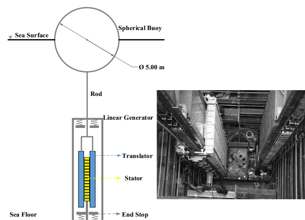
Fig. 1. Schematic of the heaving point absorber concept and photo of the reference generator in AWS pilot plant [4]
