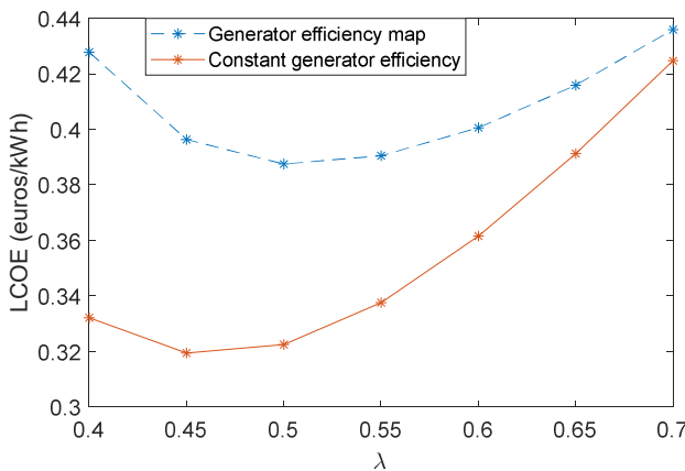
Fig. 7. The LCOE as a function of the scale factor of the generator
