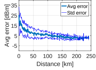
Figure 2: Error between Friis model and measurements.
