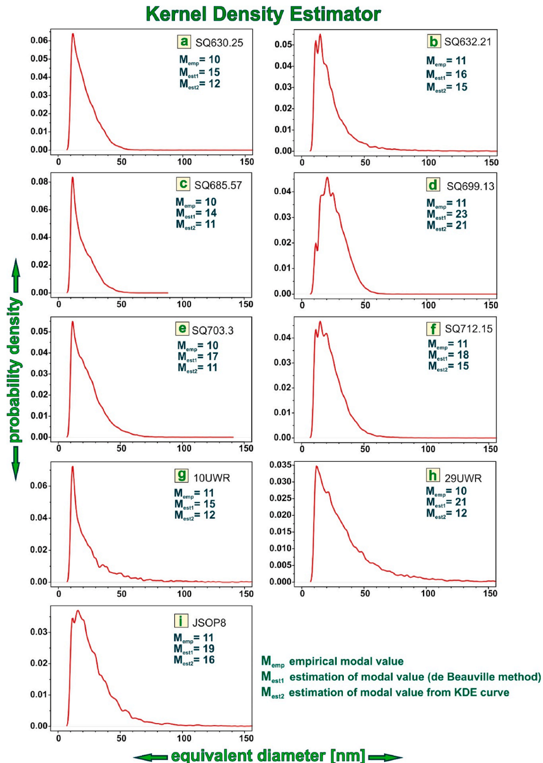
Fig. 16. Kernel density estimators (bandwidth equals 1) based on the measurements of diameters of pores visible in SEM BSE images. All the KDE curves indicate the unimodal shape, however, some secondary peaks may be linked with different types of porosity, i.e. organic matter porosity, cracks, or clay mineral aggregates. Pores greater than 150 nm were omitted because of their negligible meaning and for better clarity of the graphs.
