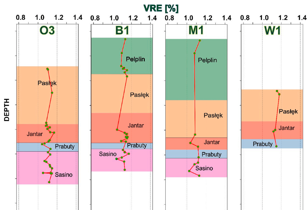
Fig. 10. Vertical changes of organic matter reflectance (measured as solid bitumen reflectance SBR o and recalculated into vitrinite equivalent VRE) in examined sections of wells O3, B1, M1, and W1.
