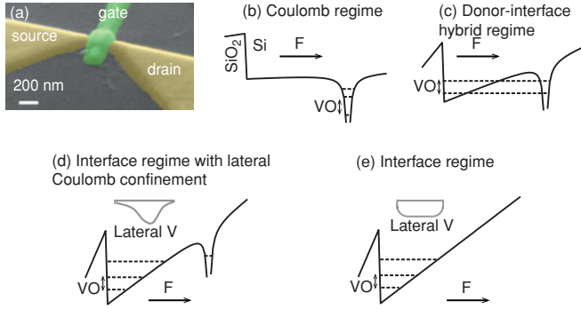
FIG. 1. (Color online) (a) SEM image of a FinFET device used in the experiments. (b)–(e) Schematic of the various confinement regimes showing the vertical confinement potential near the oxide interface. (b) is a donor bound Coulomb confinement regime at low E field. (c) is a hybrid confinement regime between the donor and the interface well realized at higher E fields when the two wells are lined up in energies and are strongly tunnel coupled. (d) is an interfacial confinement regime realized at even higher fields, but laterally bound by the donor Coulomb potential. (e) is a QD-like confinement regime realized at strong E fields for device samples without any influence of the donor. The lateral confinement is provided by the residual barriers in the access regions. The insets show schematics of the lateral confinement potential in (d) and (e).
