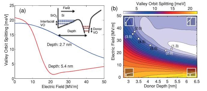
FIG. 2. (Color online) (a) Tight-binding calculations of VO splitting in Si in the presence of a single As donor as a function of field for two donor depths. The inset shows a 1D schematic of the confining potential with the donor. (b) VO splitting as a function of donor depth and electric field obtained from TB. The white markers show the measured VO splitting for six device samples extracted from the measurements of Ref. 19. The measured VO energy in milli-electron-volts is shown in parentheses beside each data point.
