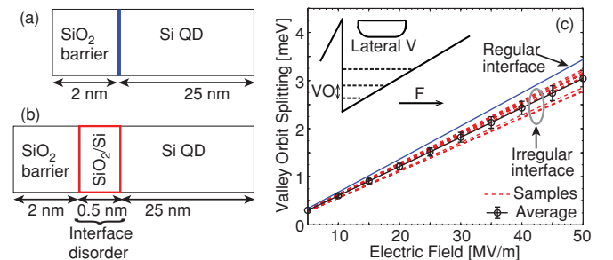
FIG. 4. (Color online) (c) TB simulations of VO splitting as a function of the vertical field for an ordered (a) and disordered (b) surface.
