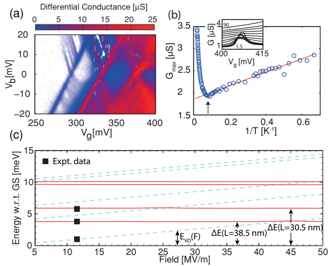
FIG. 3. (Color online) (a) Conductance vs gate and bias voltage plot for a device without the influence of a donor [confinement regime Fig. 1(e)] showing blocked diamond region and tunneling through the QD states, characteristic of Coulomb blockade. (b) Inset: Measured conductance data of the device as a function of gate voltage and temperature ( T ) between 1.5 and 90 K. The temperature steps are not all equal. Main plot: The peak maxima (extracted from the inset) vs 1/T , showing a crossover from single level transport (linear regime) to classical transport at higher T . (c) Calculated spectrum of a MOS QD relative to the ground state, with lateral dimensions of 30.5 \text{ nm} \times 38.5 \text{ nm} , as a function of the vertical electric field, showing VO split states matched to the measured values.
