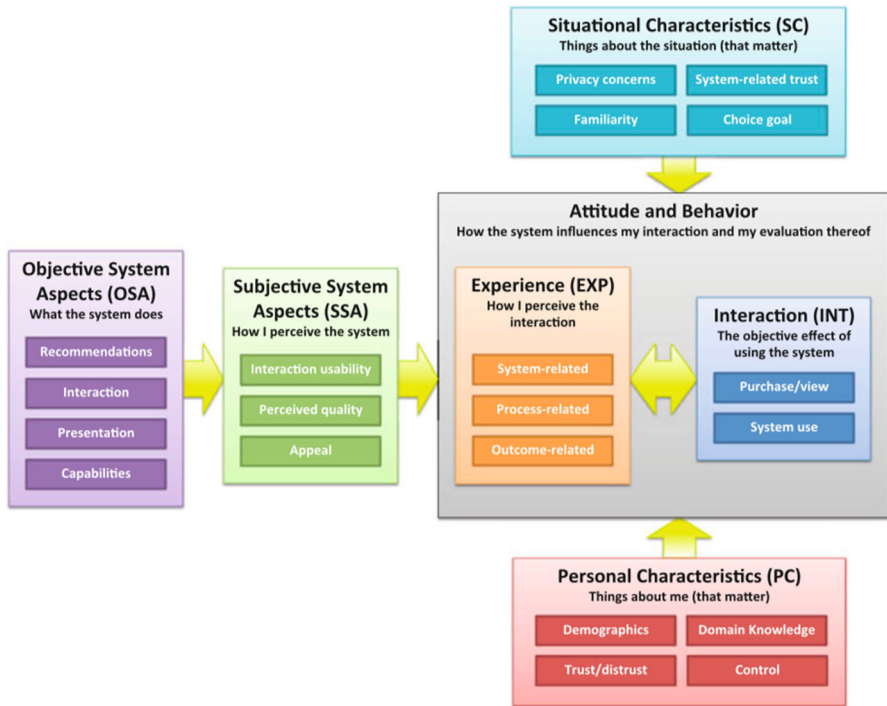
Fig. 6 The conceptual model in a framework for the user-centric evaluation of recommender systems (Knijnenburg et al. 2012)
