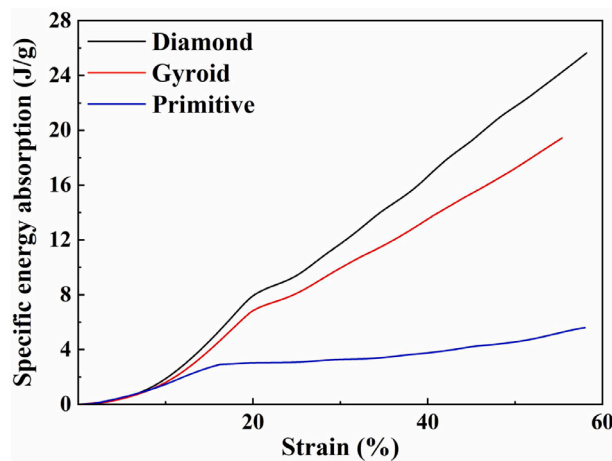
Fig. 7. Energy absorption diagram of TPMS.
