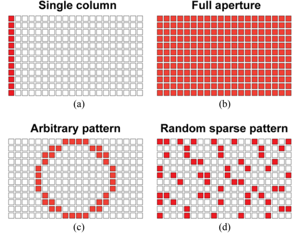
Fig. 5. Element-selection modes supported by the ASIC: (a) single-column selection; (b) full-aperture selection; (c) selection of arbitrary sets of elements; (d) pseudo-random element selection.
