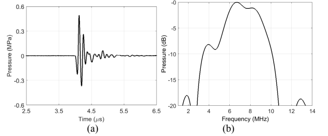
Fig. 16. Measured acoustic pressure recorded with a hydrophone: (a) time-domain waveform, (b) frequency spectrum.
