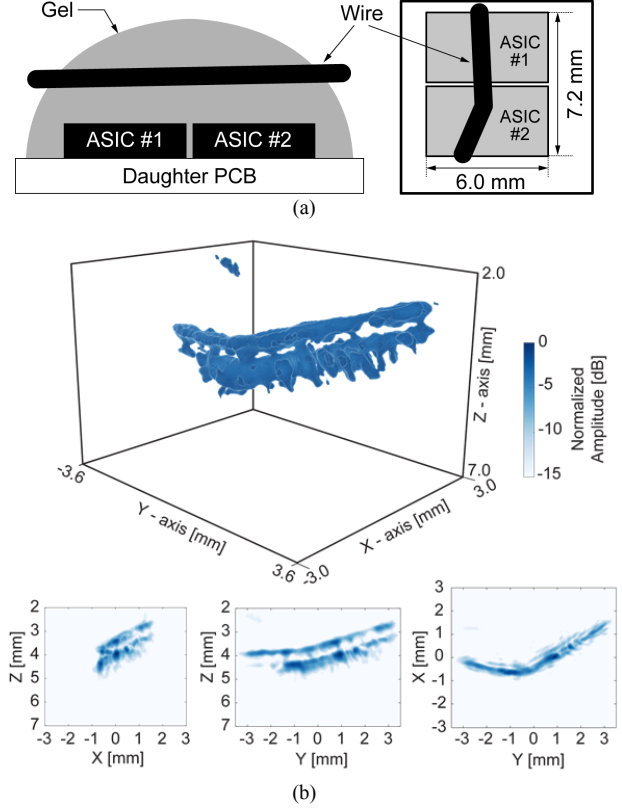
Fig. 18. (a) Setup with two ASIC tiled side-by-side for a 3D imaging experiment; (b) reconstructed volumetric images along with maximum projections.
