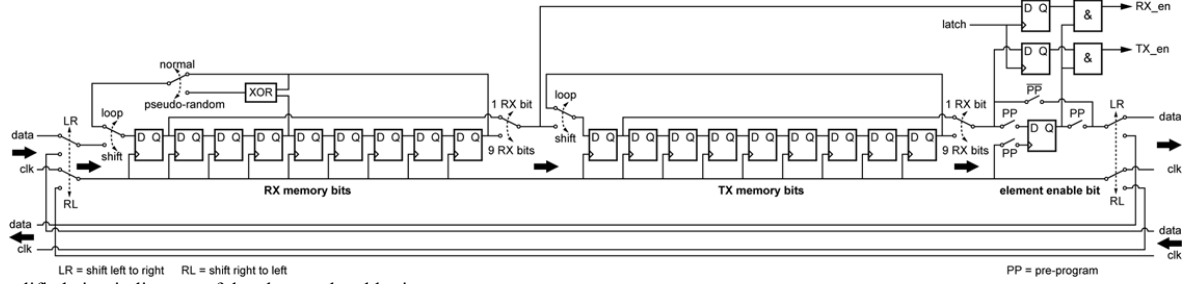
Fig. 9. Simplified circuit diagram of the element-level logic.
