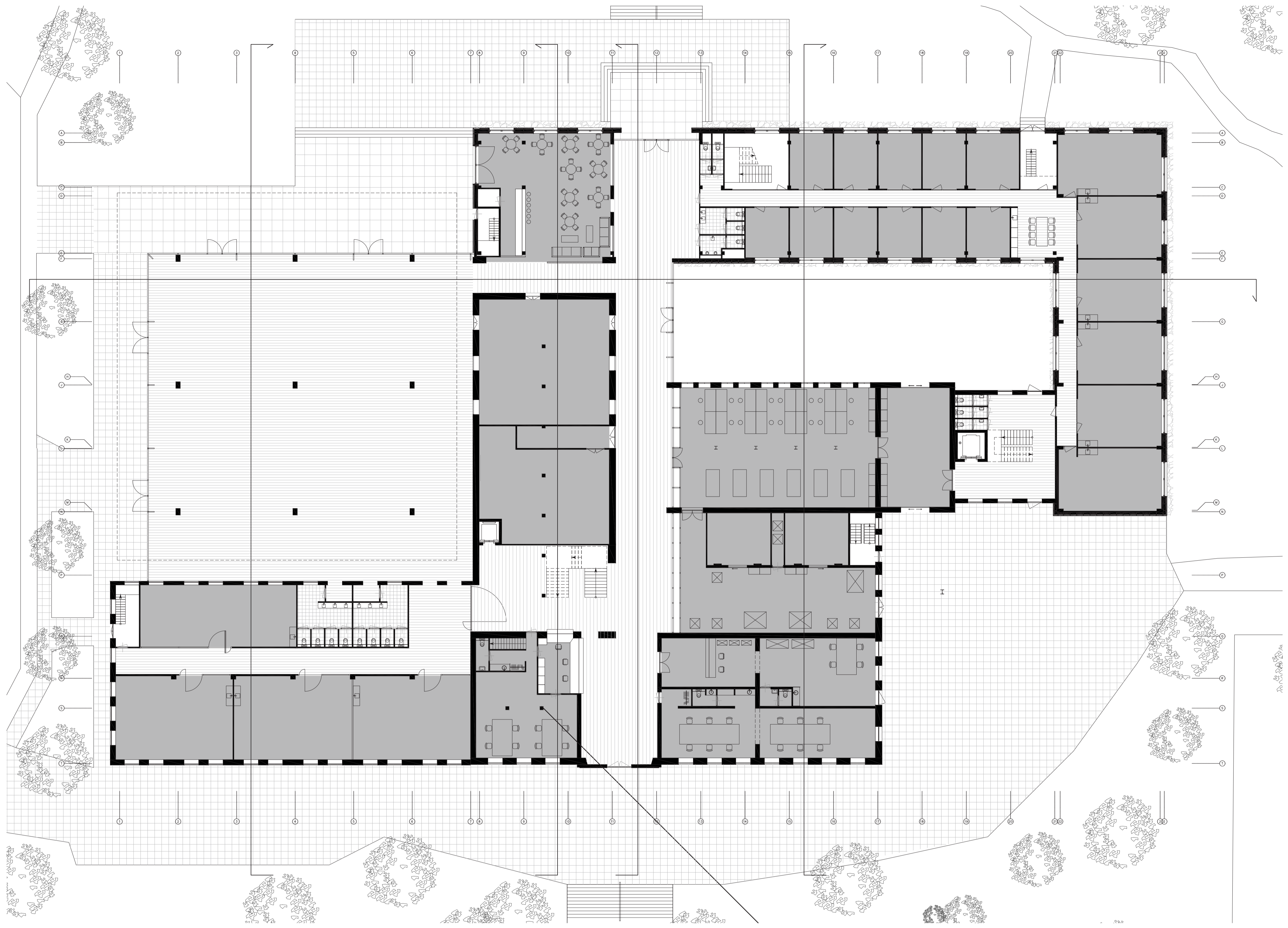
begane grond 1:200
