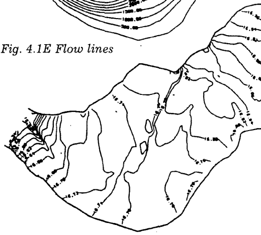
Fig. 4.1F Piezometric heads
