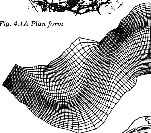
Fig. 4.1B Curvilinear grid
