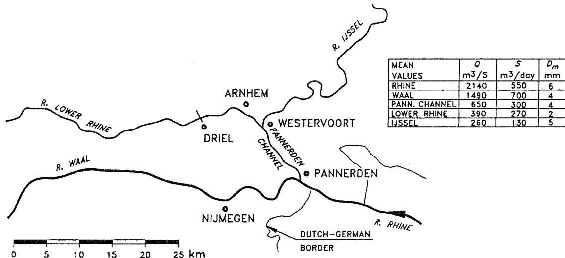
Fig. 3.8 Bifurcations at Pannerden and Westervoort, the Netherlands
