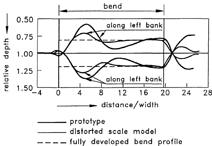
Fig. 3.1 Scale effect in bend topography (Struiksmas, 1986)
