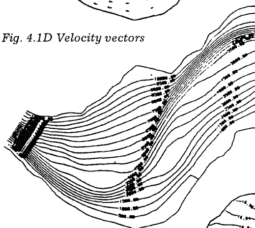
Fig. 4.1E Flow lines
