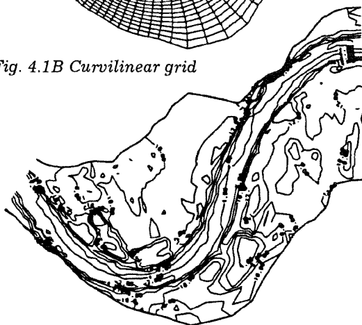
Fig. 4.1C Bed elevations
